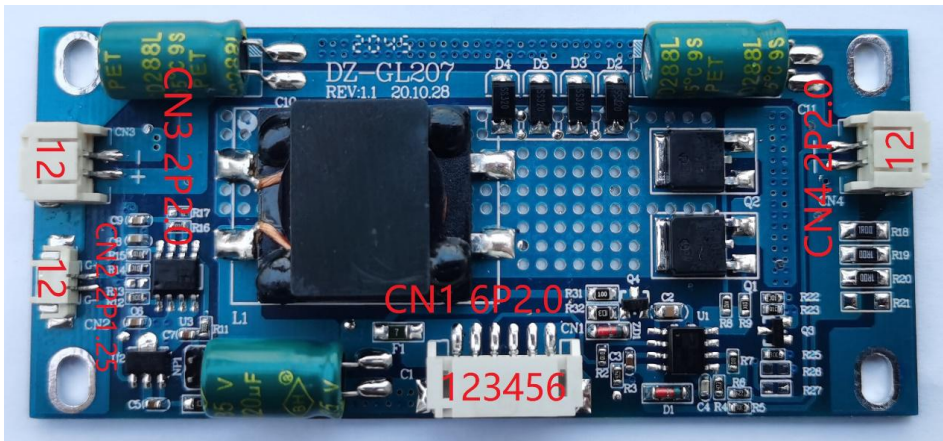
图 1-2 General view
