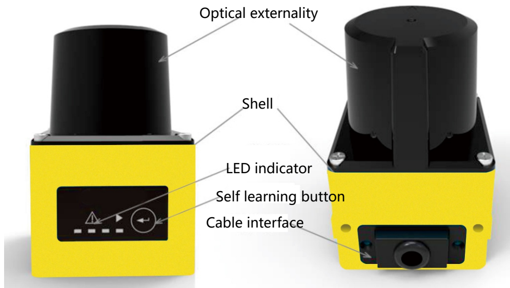
Figure 2-1 DADI appearance 1
