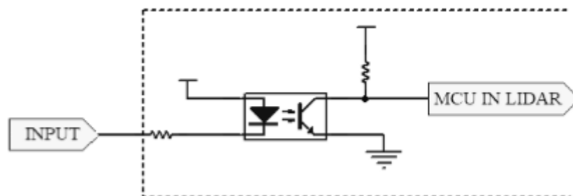
Figure 5-9 input circuit
