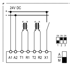
5. Dual-channel 2-wire edge/mat (no resistance) safety input, with manual reset
