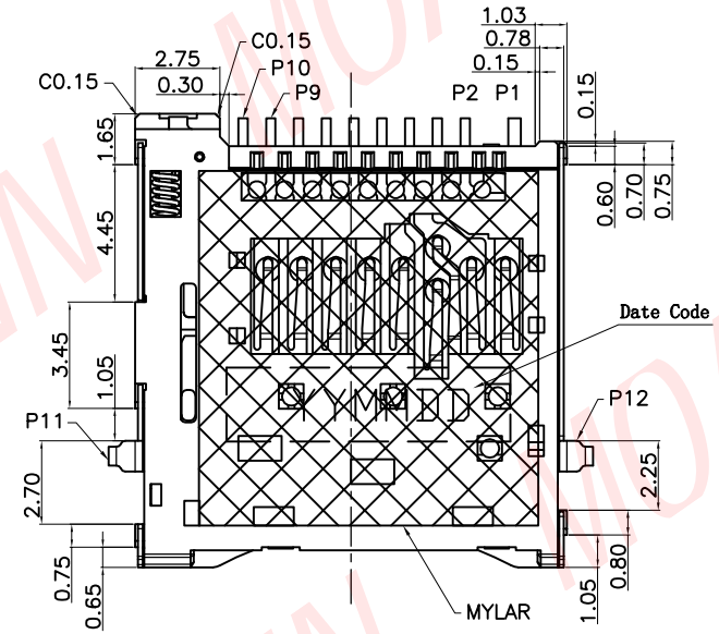
BOTTOM VIEW (CONNECTOR) TOP VIEW (SYSTEM)
