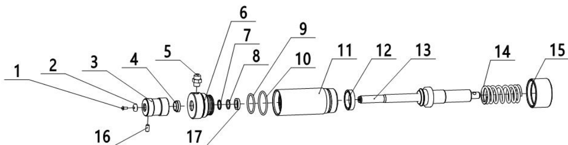
#98002 hydraulic cylinder Explosive view
