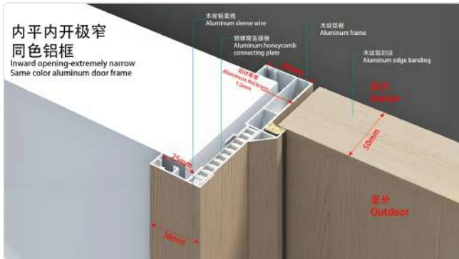
Inward opening-extremely narrow Same color aluminum door frame 内平内开极窄同色铝框
