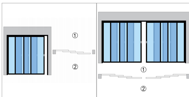
BFS2=4 Linkage 4 Doors Right Door Leat At Outside
