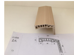
6046 Sloped line
