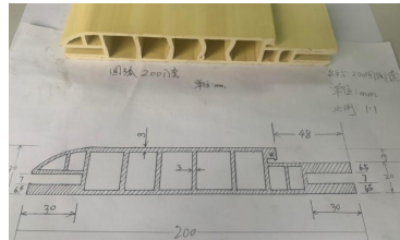
20030 curved frame
