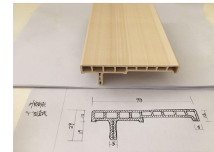
9829 T-shape line
