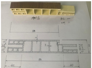
19031 Frame
