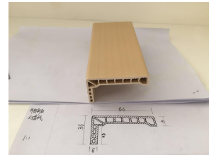
6536 Line
