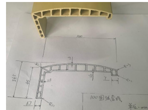
10054 Curved lines
