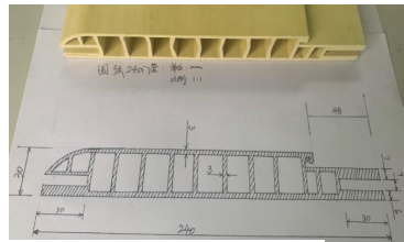
24030 curved frame
