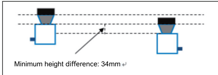
Figure 5.2 Scan plane height adjustment
