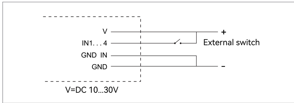
Figure 6.4 External circuit for I/O interface input terminals (floating)
