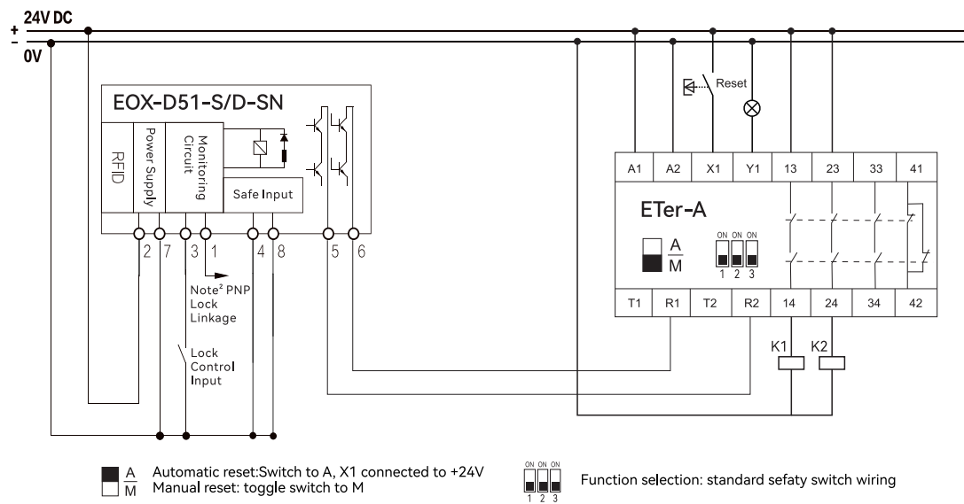
Example 3. EOX-D51-S/D-SN and safety relay ETer-A form a dual-channel configuration with manual reset and OSSD locking linkage.
