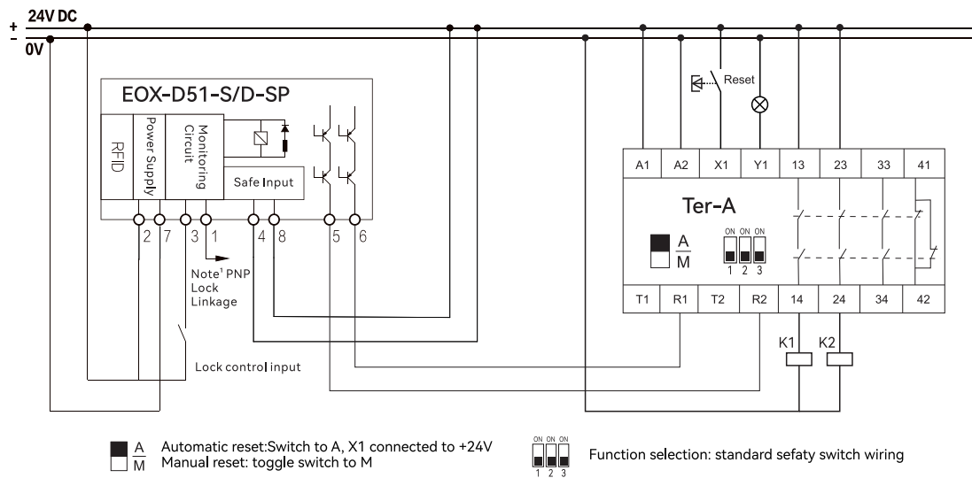
Example 1. EOX-D51-S/D-SP and safety relay Ter-A form a dual-channel system with automatic reset and OSSD locking linkage.
