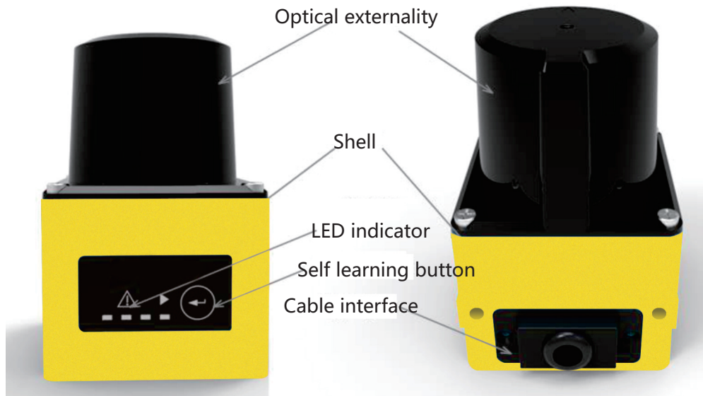
Figure 2-1 radar appearance 1
