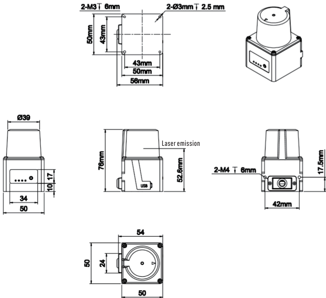
Figure 5-1 radar mechanical dimensions
