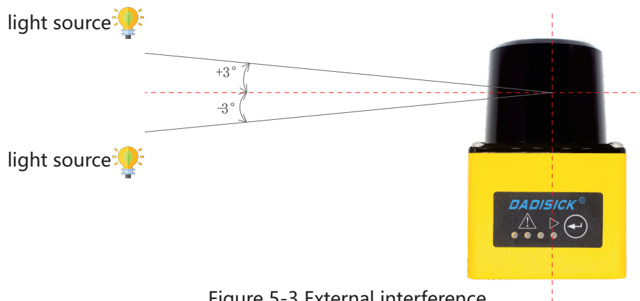
Figure 5-3 External interference
