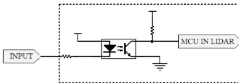
Figure 5-9 input circuit
