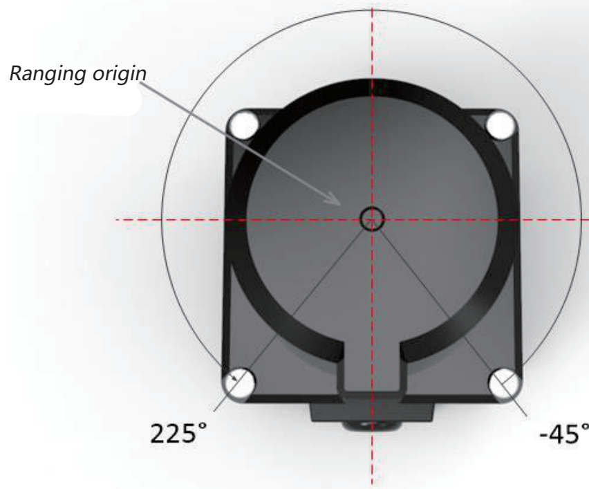
Figure 2-3 scanning angle
