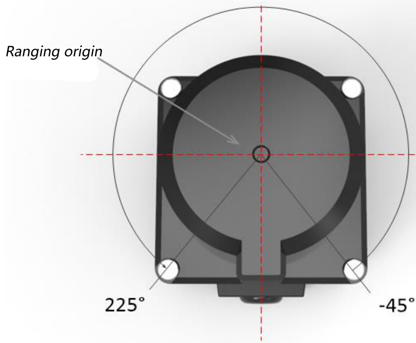
Figure 2-3 scanning angle
