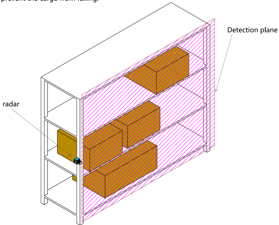
Figure 6-2 Projection detection
