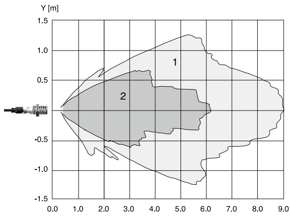
Curve 1: Flat plate 100mm x 100mm Curve 2: Round bar φ25mm ECSB30-6000 series
