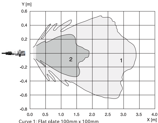
Curve 1: Flat plate 100mm x 100mm Curve 2: Round bar φ25mm ECSB30-2000 series
