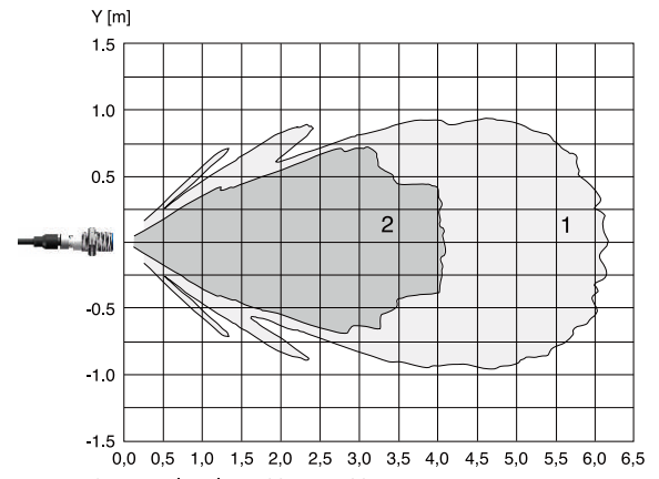
Curve 1: Flat plate 100mm x 100mm Curve 2: Round bar φ25mm ECSB30-4000 series
