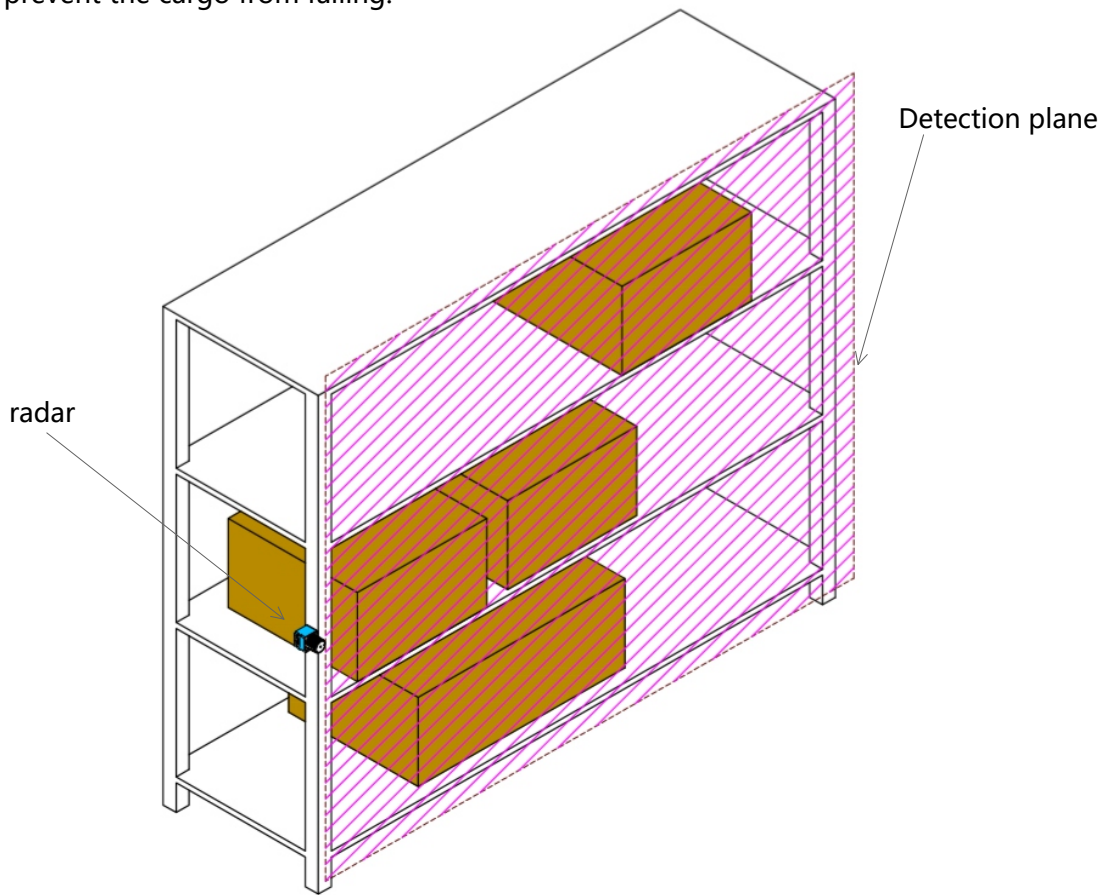
Figure 6-2 Projection detection
