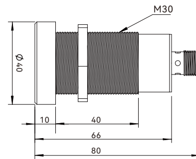
DK-CSC30-2500 series
