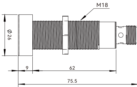
DK-CSC18-1000 series
