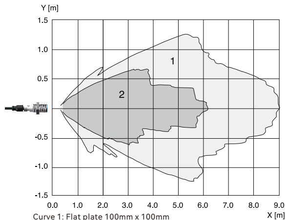
Curve 1: Flat plate 100mm x 100mm Curve 2: Round bar \phi 25mm DK-CSB30-6000 series
