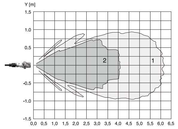
Curve 1: Flat plate 100mm x 100mm Curve 2: Round bar \phi 25mm DK-CSB30-4000 series
