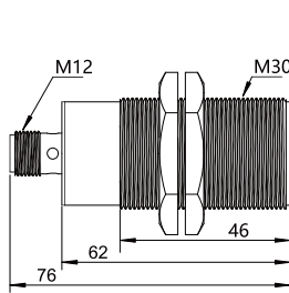
DK-CSB30-2000 series
