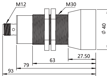
DK-CSB30-4000 series
