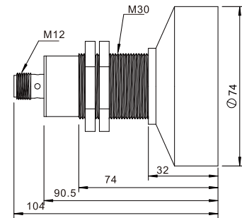
DK-CSB30-6000 series
