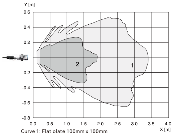
Curve 1: Flat plate 100mm x 100mm Curve 2: Round bar \phi 25mm DK-CSB30-2000 series
