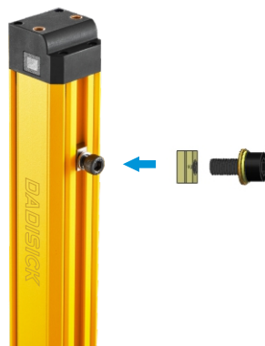
3. Installation method of convex nut (Optional accessories)
