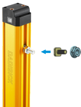
2. Installation method of T-shaped screws on the back (Original accessories)
