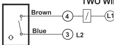
Plastic housing AC/DC 20-250V or AC 20-250V TWO WIRE-NO
