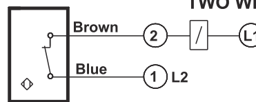
Plastic housing AC/DC 20-250V or AC 20-250V TWO WIRE-NC
