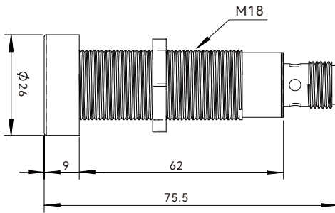
CSC18-1000 series
