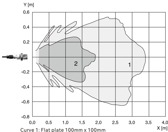
Curve 1: Flat plate 100mm x 100mm Curve 2: Round bar \phi 25 mm CSB30-2000 series
