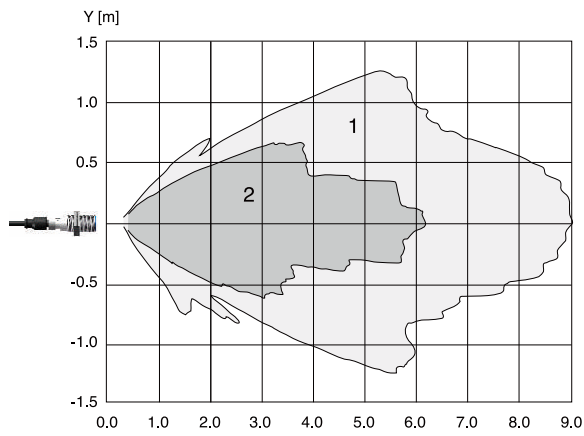
Curve 1: Flat plate 100mm x 100mm Curve 2: Round bar \phi 25 mm CSB30-6000 series
