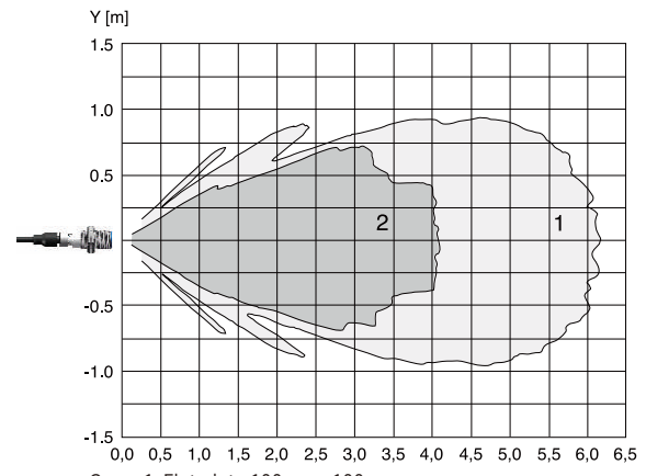
Curve 1: Flat plate 100mm x 100mm Curve 2: Round bar \phi 25 mm CSB30-4000 series
