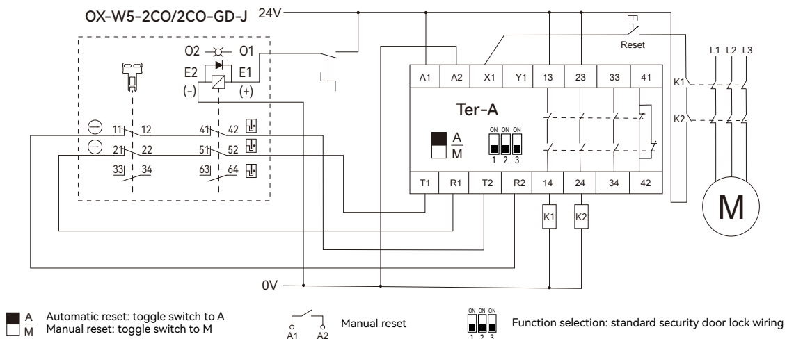
This is an example wiring diagram of OX-W5-2CO/2CO-GD-J.
