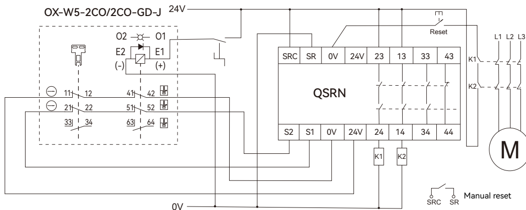
This is an example wiring diagram of OX-W5-2CO/2CO-GD-J.
