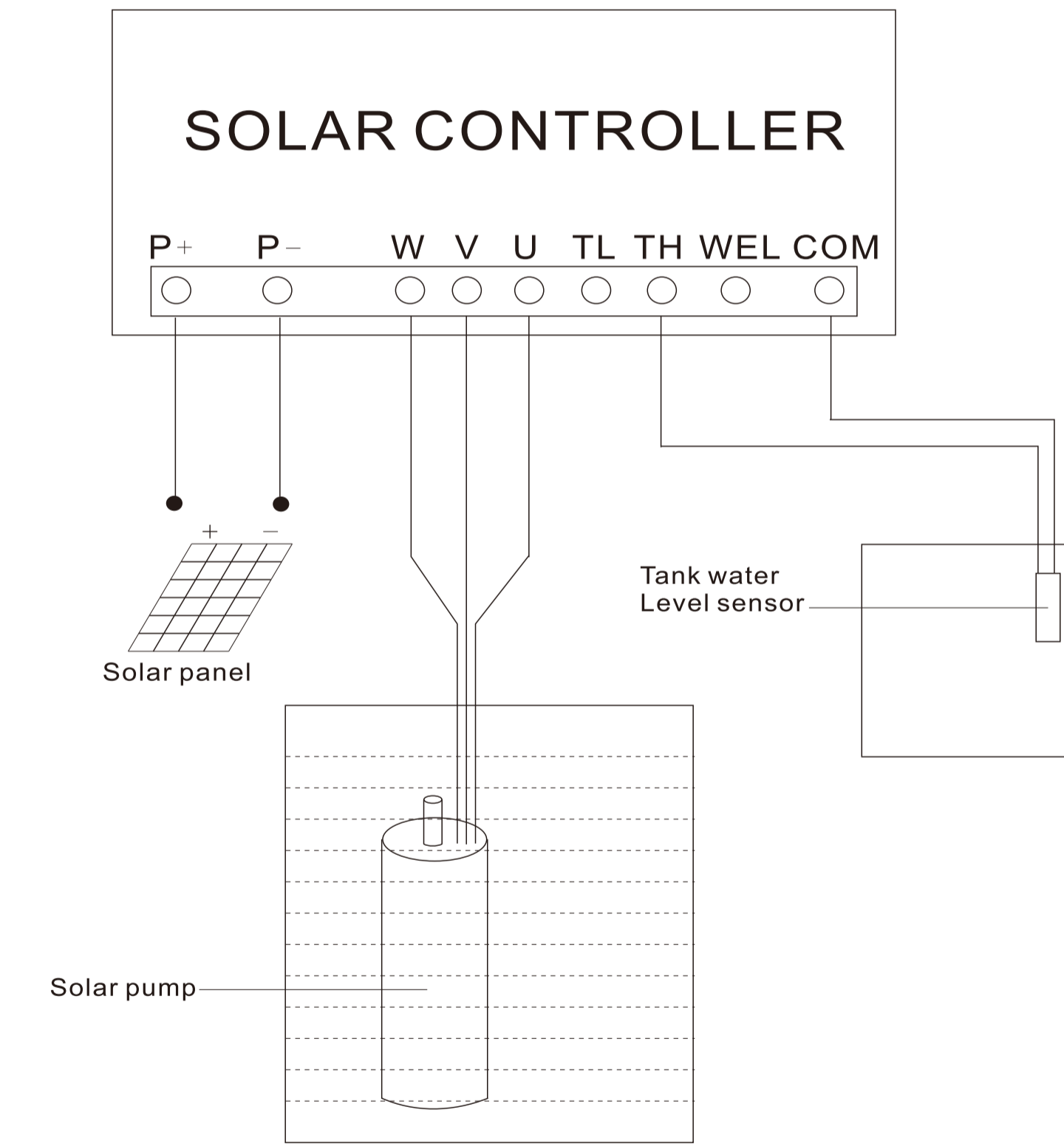
Solar Pump Controller Connection
