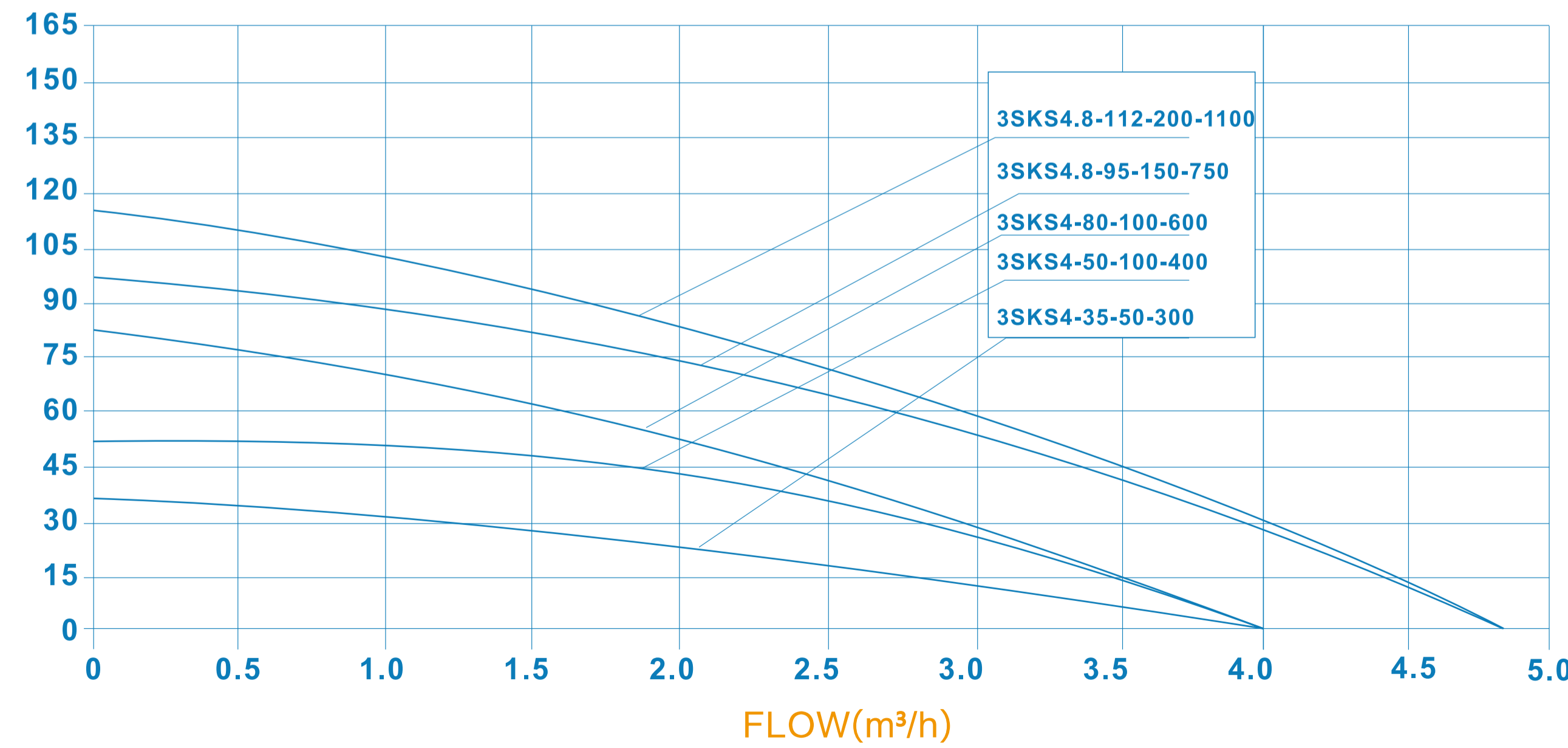
TOTAL HEAD(m)
