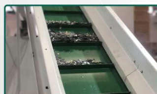
SPD200 Chip & circuit board disintegrator Final particle size: 1*1mm 2 - 3*3mm 2 Working capacity: 5-10 kg per hour
