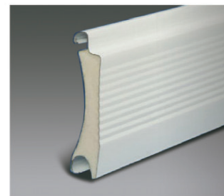
Name: 95mm foam slat Thickness: 25mm Weight: 10.0Kg/m 2 Maximum width: 8.0m Maximum height: 6.5m Maximum area: 46m 2 Quantity of per meter height: 11 pcs Material: 0.45 mm galvanized steel plate Color: White, Beige, Grey (Other color can be made upon customer's request.) Pattern: unperforated
