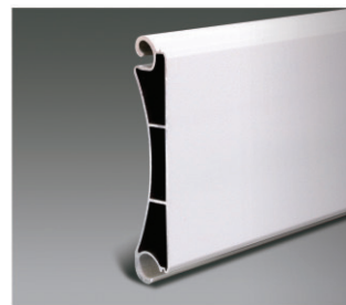
Name: 120 double layer slat for hurricane Thickness: 25.5mm Weight: 12.0Kg/m 2 Maximum width: 9.0m Maximum height: 8.0m Maximum area: 25m 2 Quantity of per meter height: 8 pcs Surface treating: powder coating Color: White, Beige, Grey (Other color can be made upon customer's request.) Pattern: unperforated
