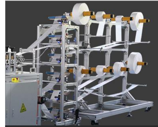
MATERIAL RACK AND INFLATABLE SHAFT
