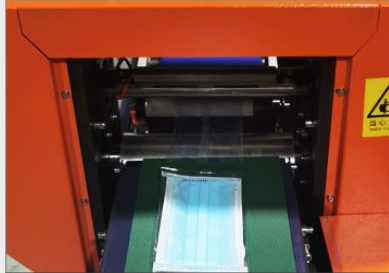
ROTARY END SEAL STRUCTURE
