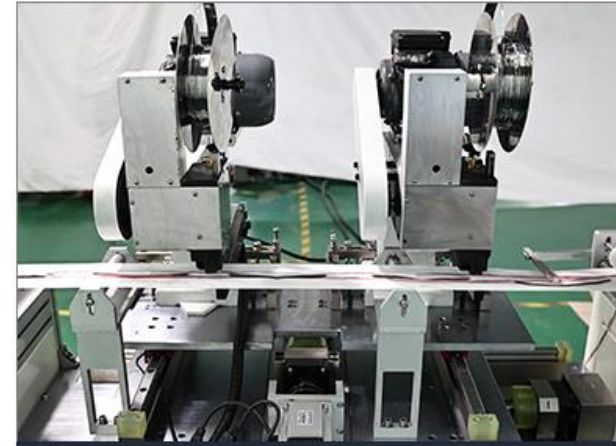
STAPLING HEADBAND
