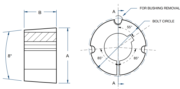
No. 1008-3030 Bushings
