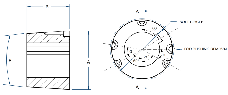
No. 3535-5050 Bushings
