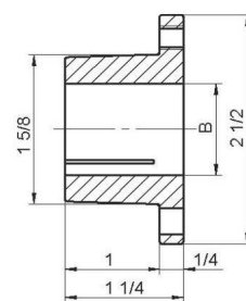
"H" Bushings
