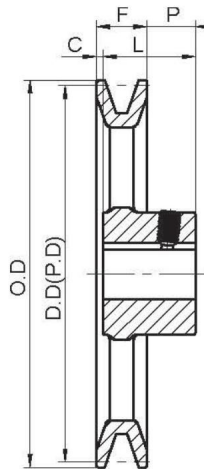
Single Groove Sheaves for "4L" or "A" Belts and "5L" or "B" Belts
