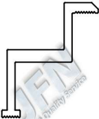
Section of Side Lock Block
