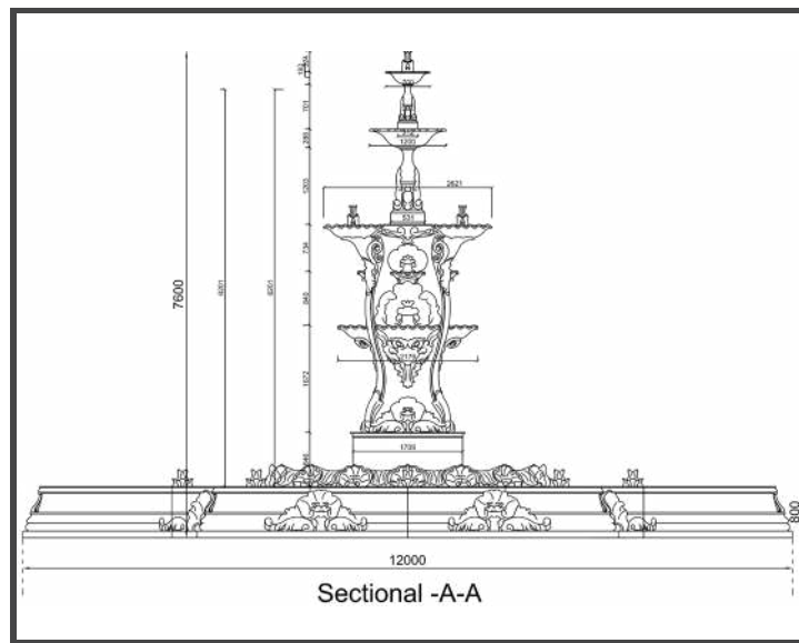
CAD Drawing
