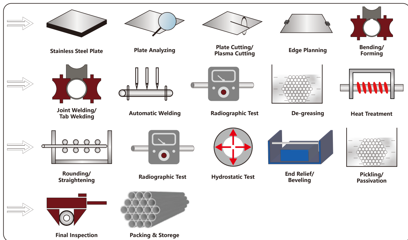
Single Formed Ss Welded Pipes Production Process Diagram
