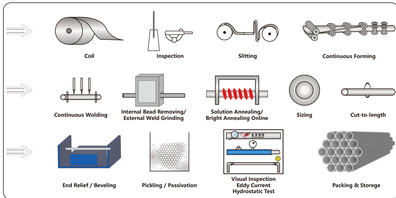
Continuous Formed Ss Welded Pipes Production Process Diagram
