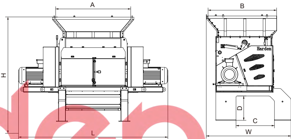
SM2200R/SM3000R Outline Drawing
