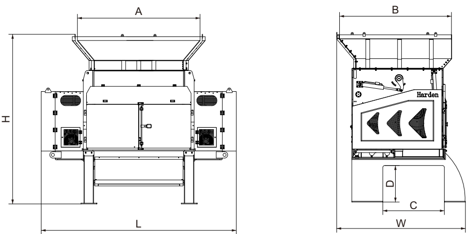
SM2200/SM3000 Outline Drawing
