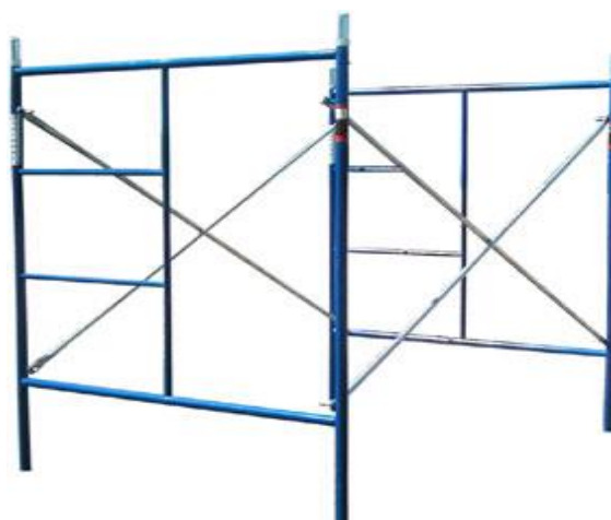
6'4"X5'FRAMES&BRACE 7'X4'(124.40LBS)
