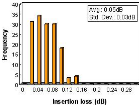
MM 62.5/125um Insertion Loss
