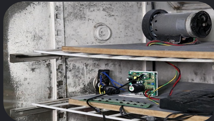
High & low temperature test chamber
