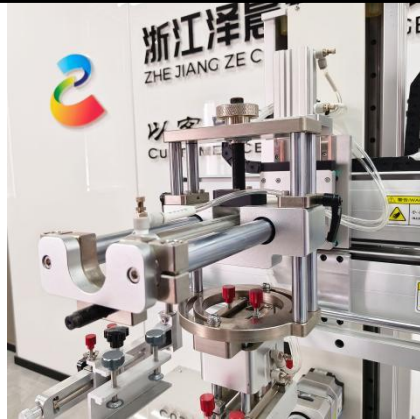
Print head details
