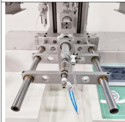
Tooling Fixtures
