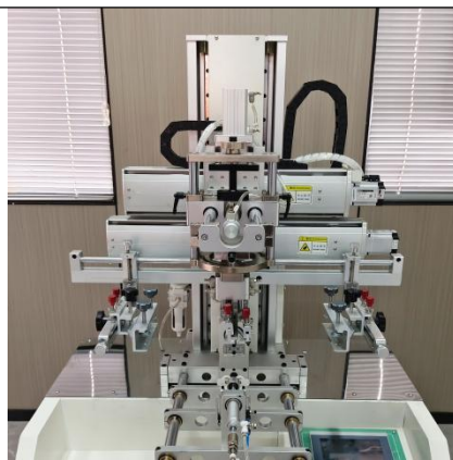
Seal head and main beam 2
