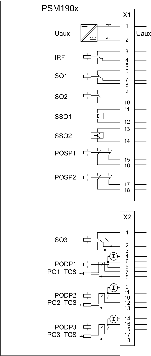
Figure 44: PSM190x module
