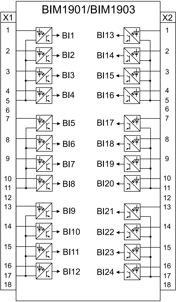
Figure 43: BIM1901/BIM1903
