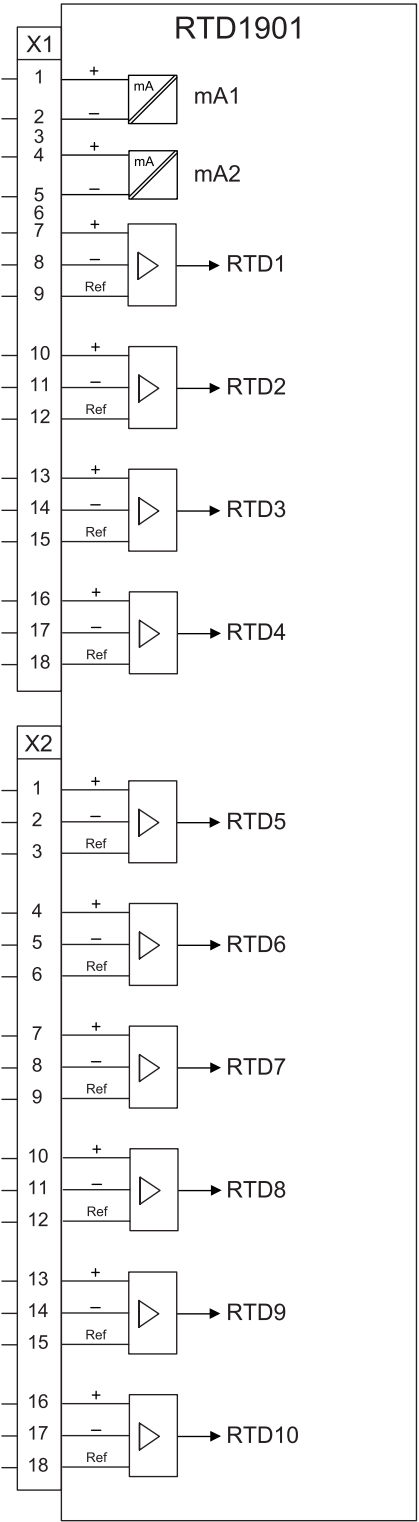
Figure 45: RTD1901 module
