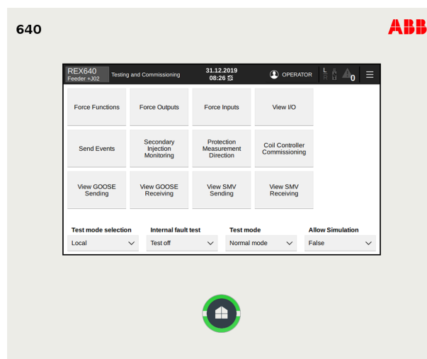
Figure 10: Test and commissioning support in the local HMI
