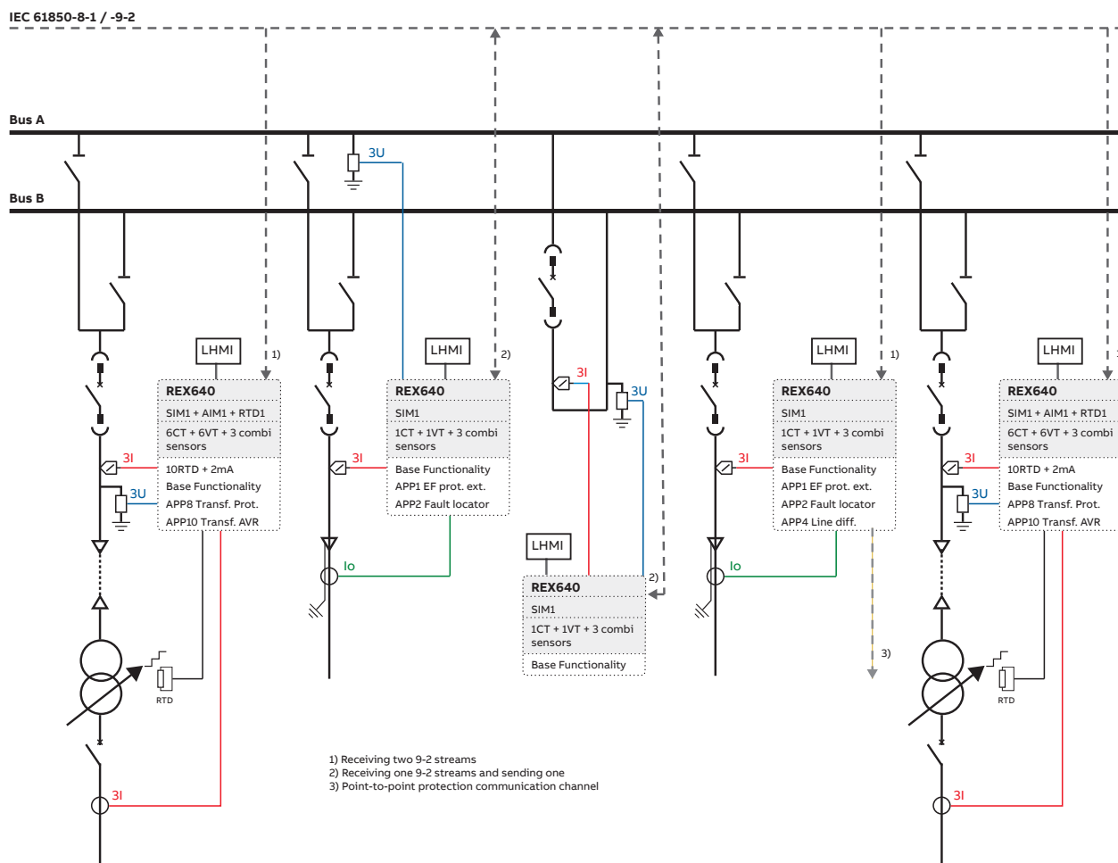
Figure 21: Digital switchgear application
