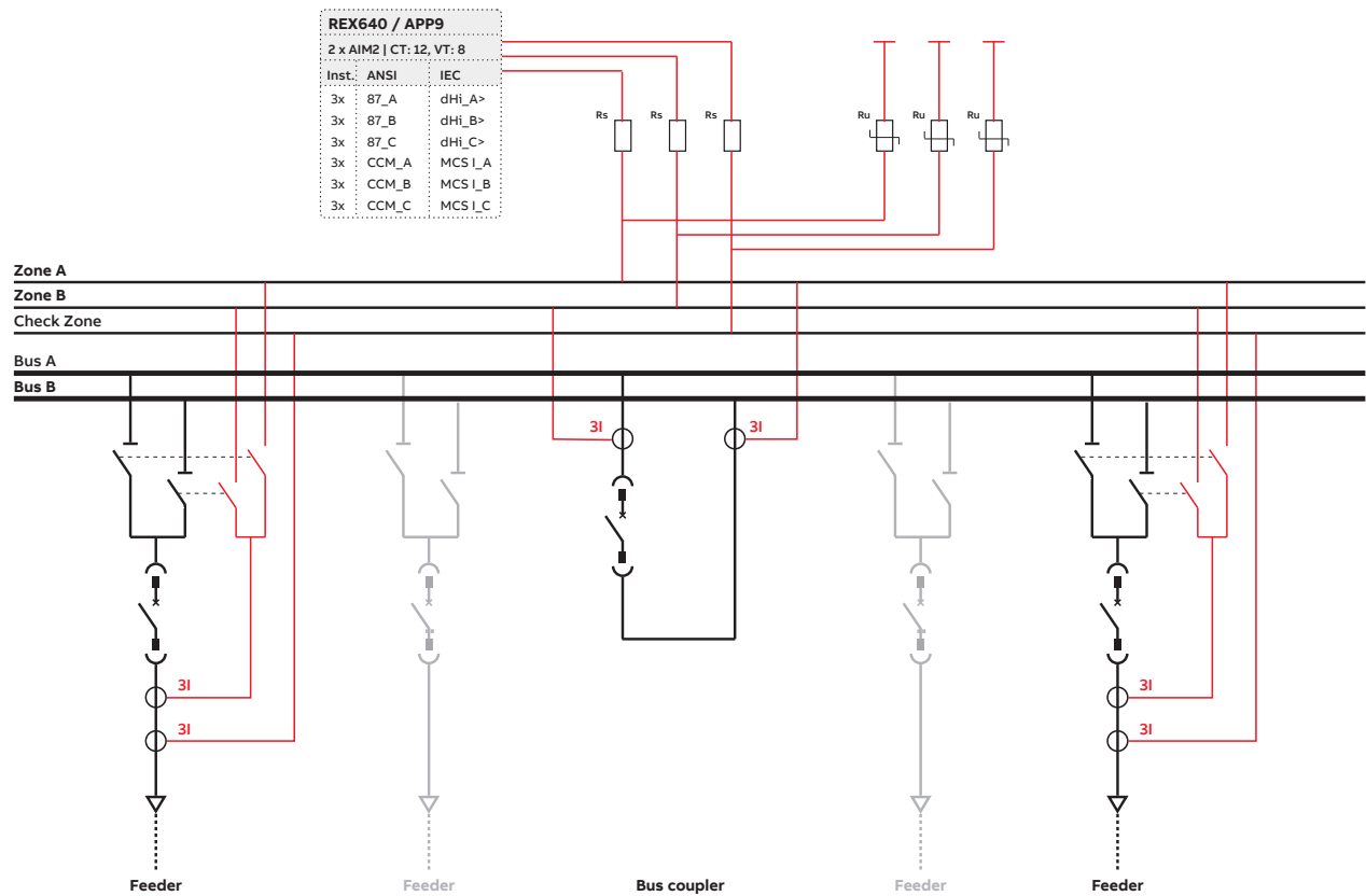
Figure 18: Busbar protection application
