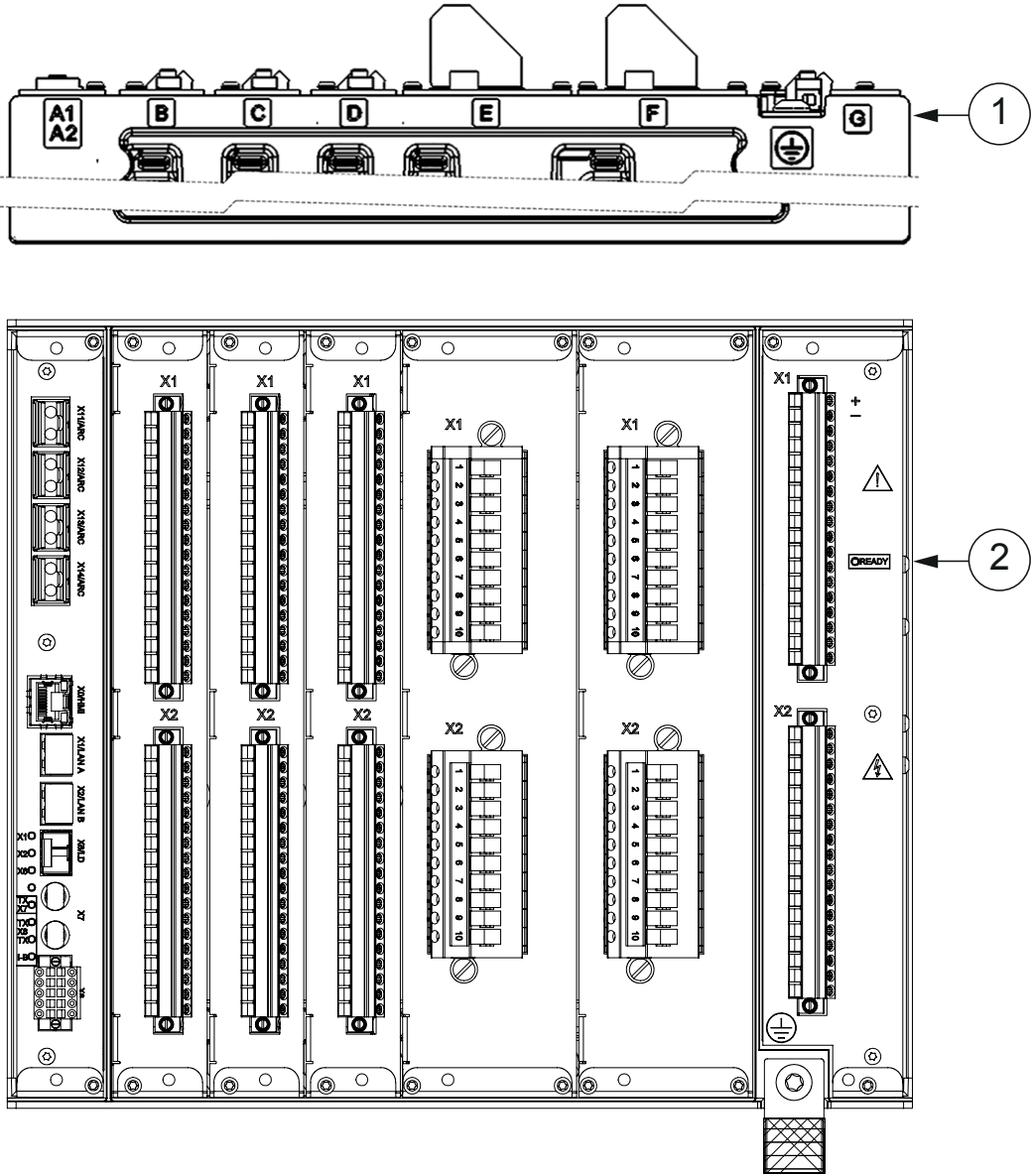
1 Slot markings in enclosure (top and bottom) 2 Ready LED
