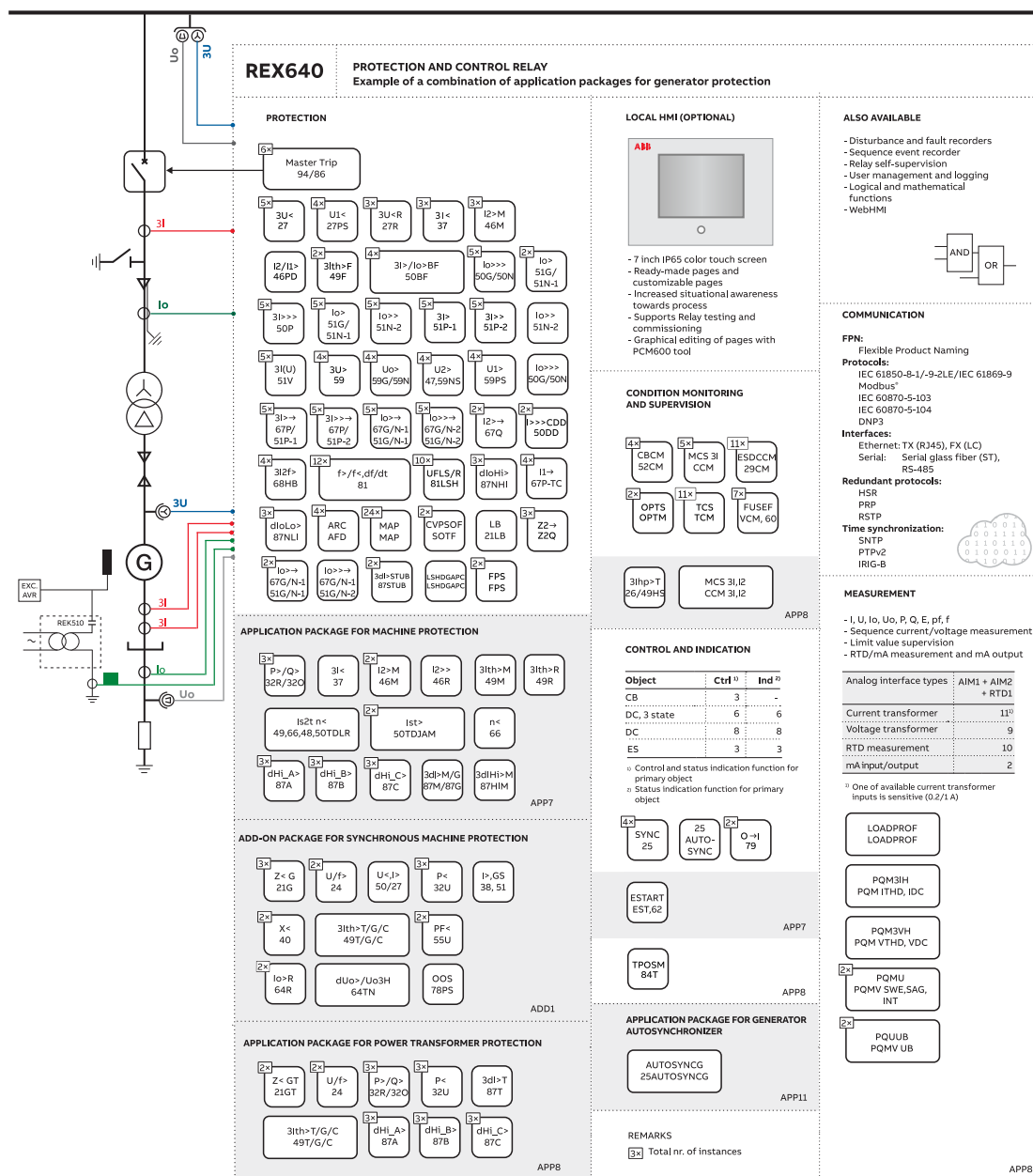
Figure 20: Generator application
