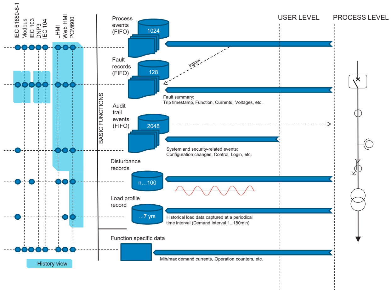
Figure 27: Event recording
