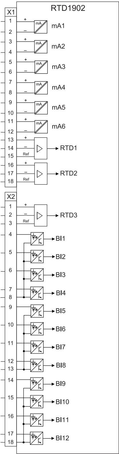
Figure 46: RTD1902 module
