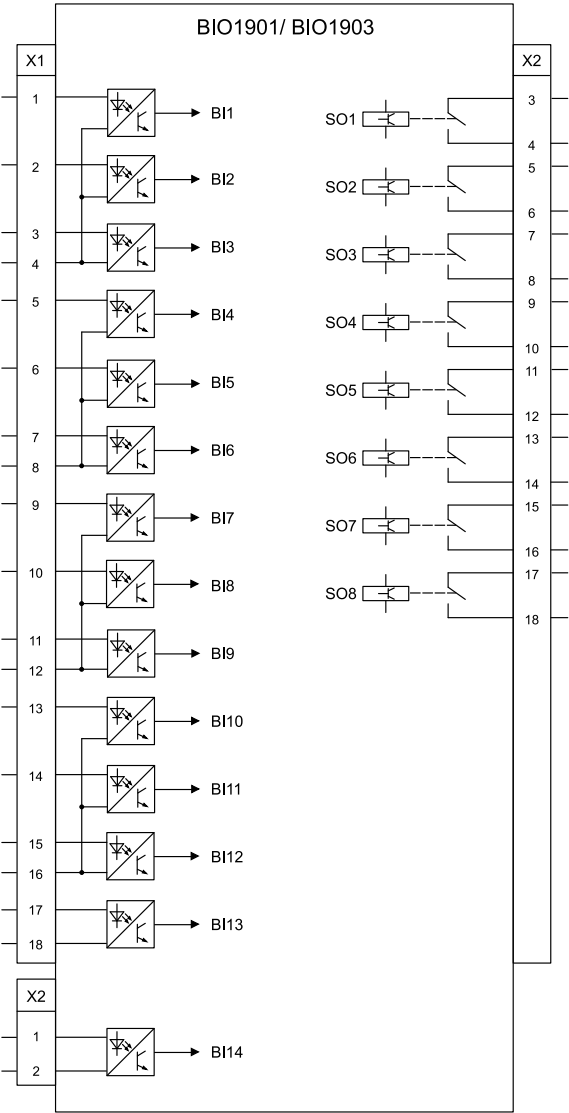
Figure 41: BIO1901/BIO1903 modules
