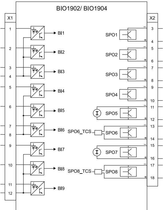
Figure 42: BIO1902/BIO1904 modules
