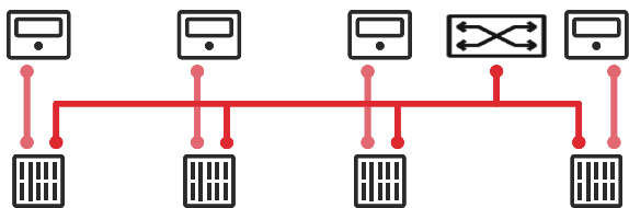
Figure 4: Local HMIs connected directly to the relays
