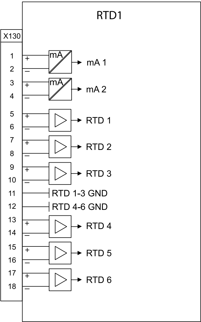
Figure 30: RTD1 module
