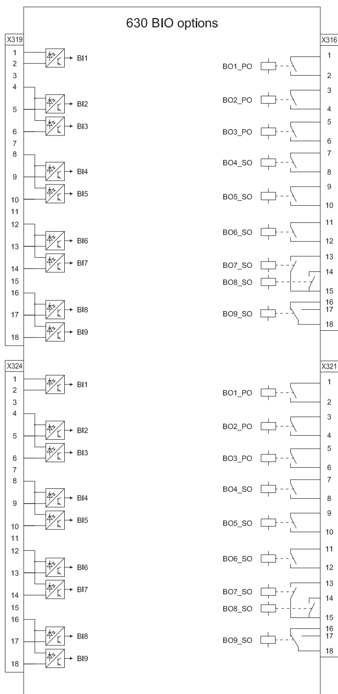
Figure 11. Terminal diagram for optional binary input/output modules for RET630 4U variant
