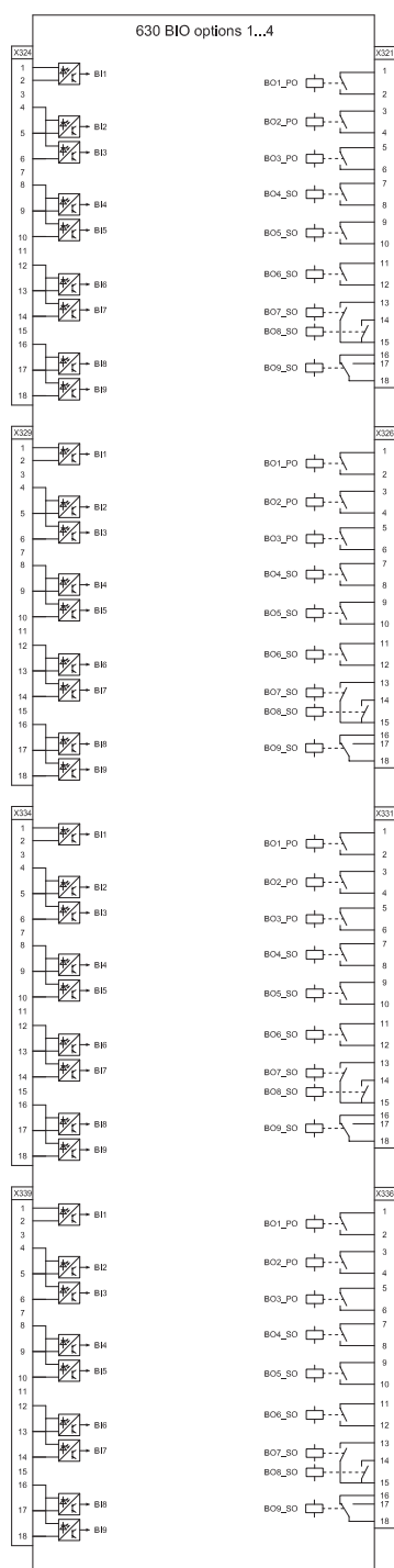
Figure 13. Terminal diagram for optional binary input/output modules for RET630 6U variant
