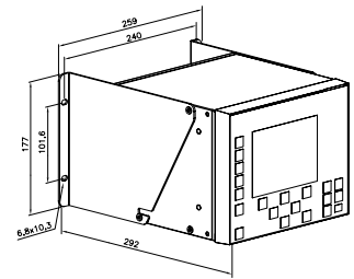
Figure 7. Wall mounting
