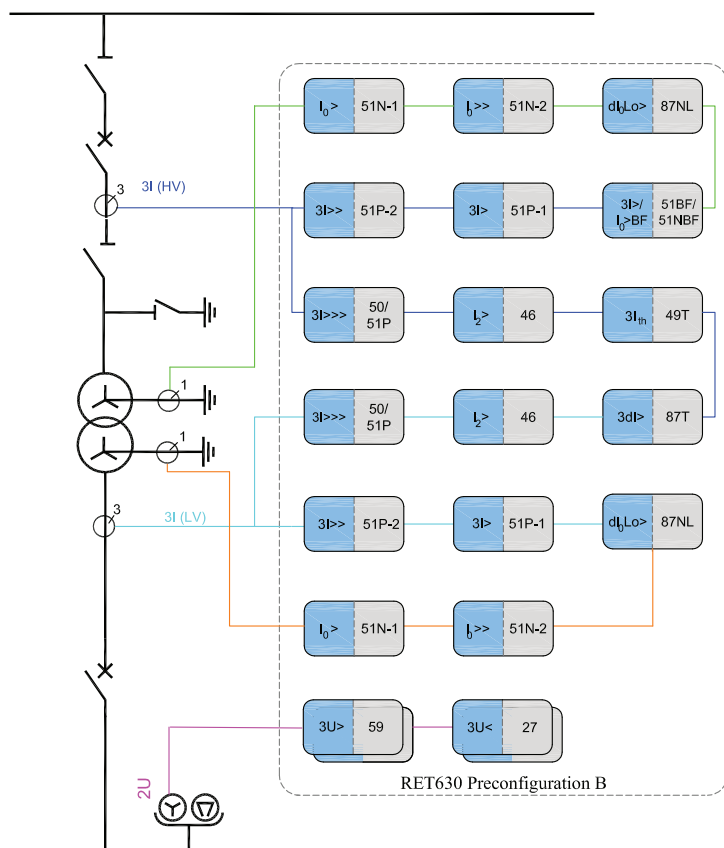
Figure 3. Protection function overview of preconfiguration B
