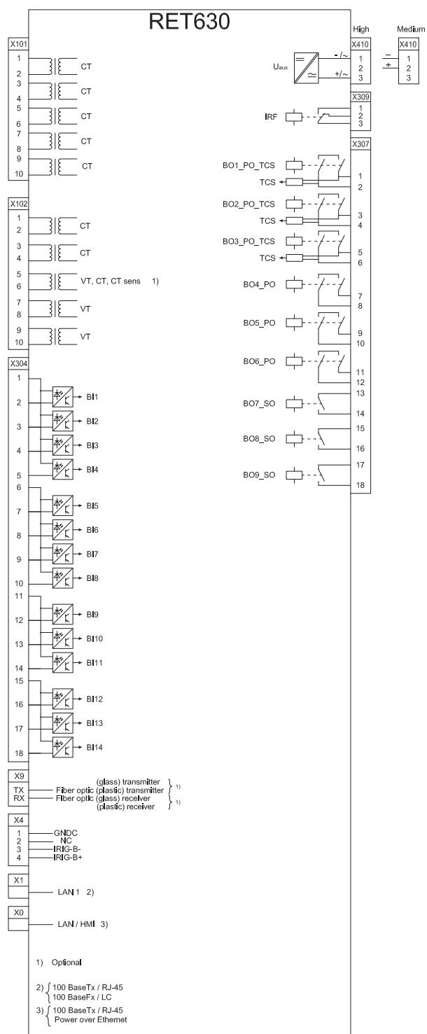
Figure 12. Terminal diagram for RET630 6U variant
