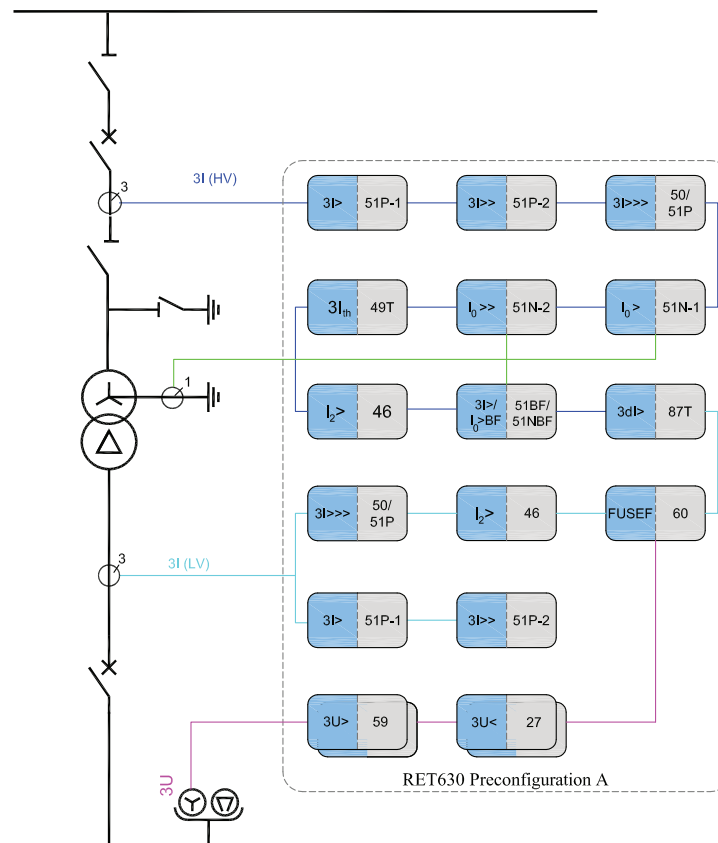
Figure 2. Protection function overview of preconfiguration A
