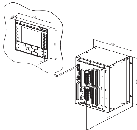
Figure 8. 6U half 19" unit wall mounted with two mounting brackets and detached LHMI
