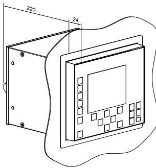
Figure 5. Flush mounting
