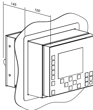
Figure 6. Semi-flush mounting
