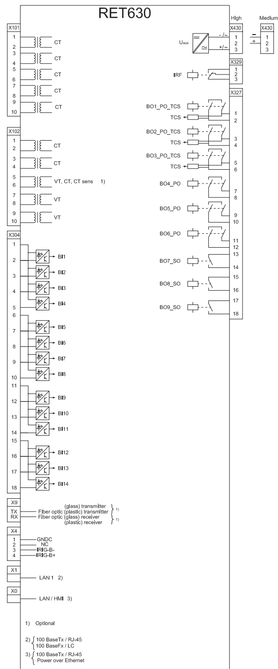
Figure 10. Terminal diagram for RET630 4U variant
