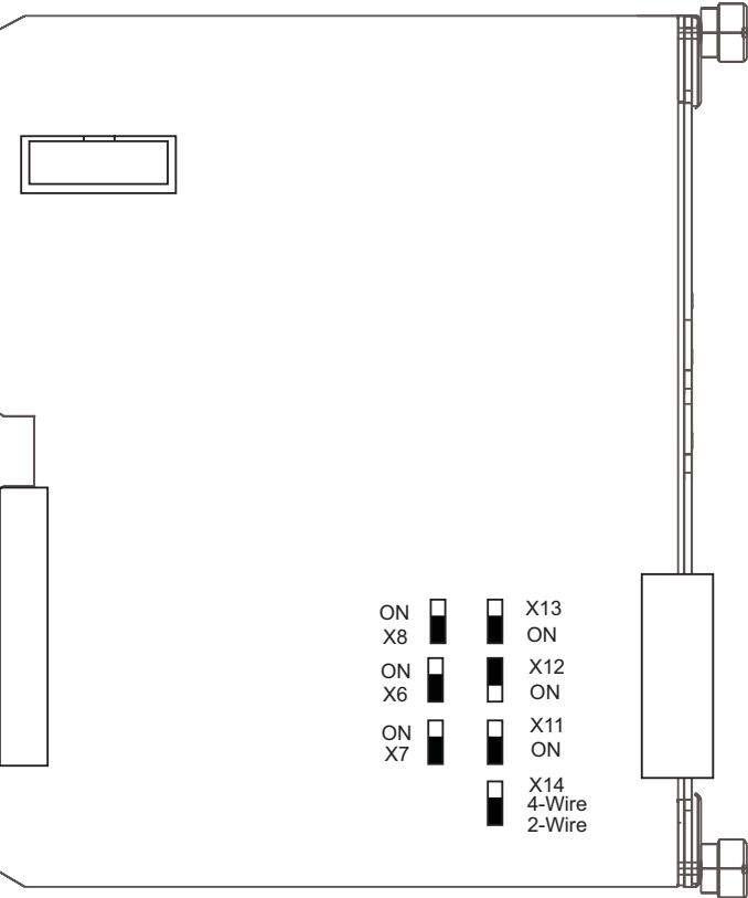
Fig. 5.2.2.-3 Jumper location on the DNP 3.0 communication module
