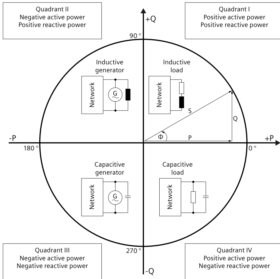
Figure 2-10 Quadrant in the quality bits
