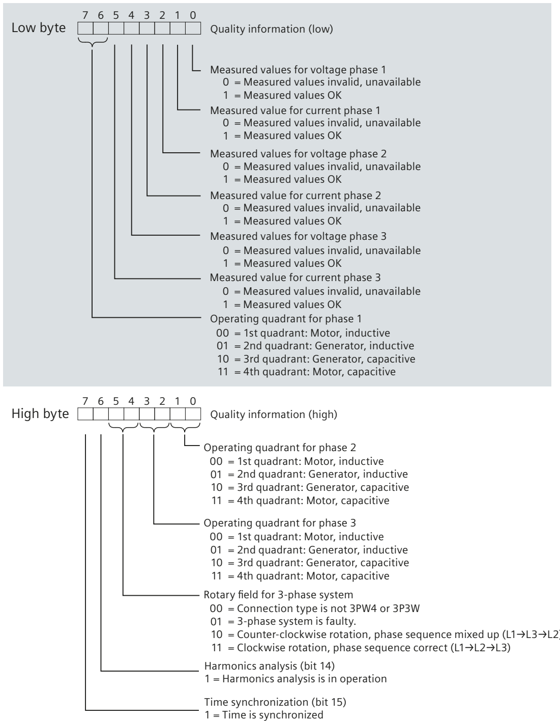
Figure 2-9 Quality information for low and high byte of the measured value ID 65503
