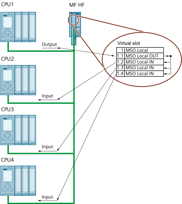
Figure 2-1 I/O data are transferred to other controllers in the same PROFINET network
