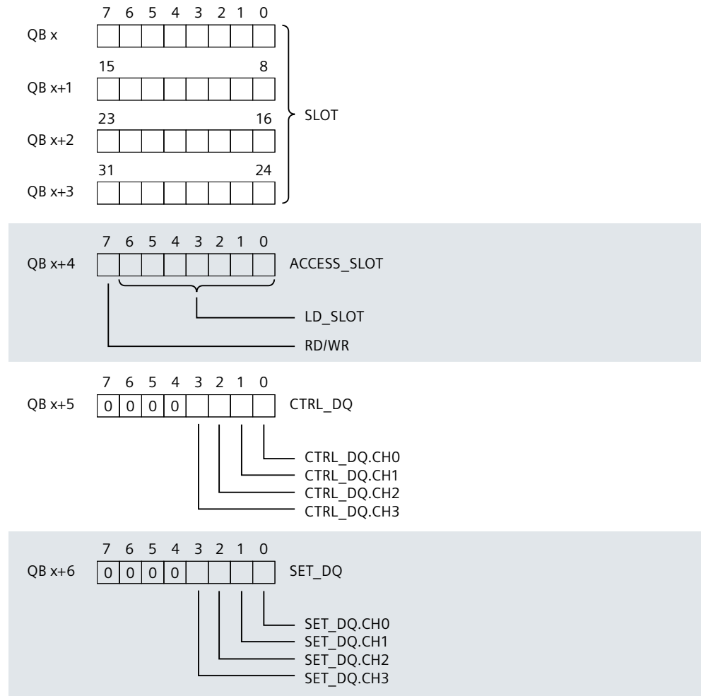
Figure 2-3 Assignment of the control interface
