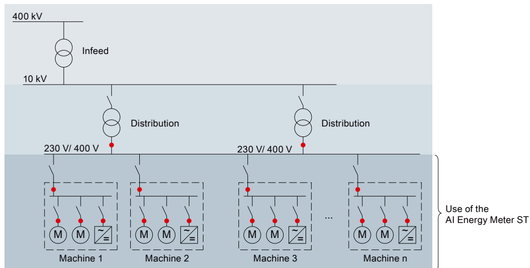
Figure 2-12 Use of the AI Energy Meter ST 400V
