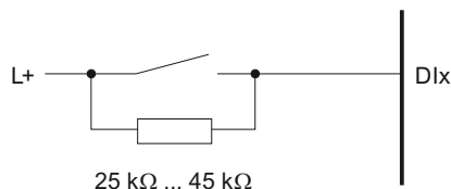
Figure 2-2 Connect mechanical encoder contact with resistor
