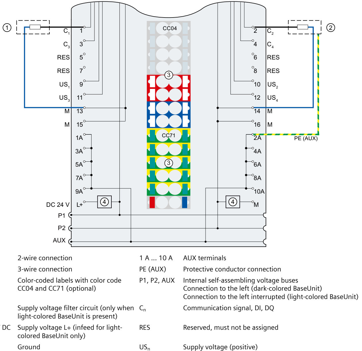
Figure 2-14 Terminal assignment for 2-wire and 3-wire connection in DQ operating mode
