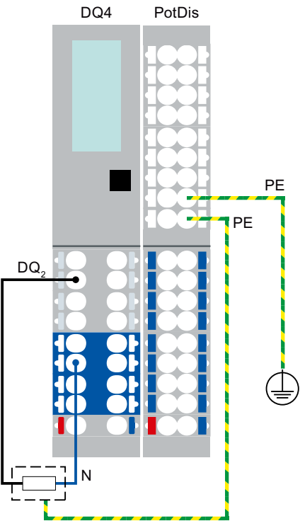
Figure 2-5 3-wire connection of actuators with potential distribution module at the digital output module DQ 4x24..230VAC/2A HF
