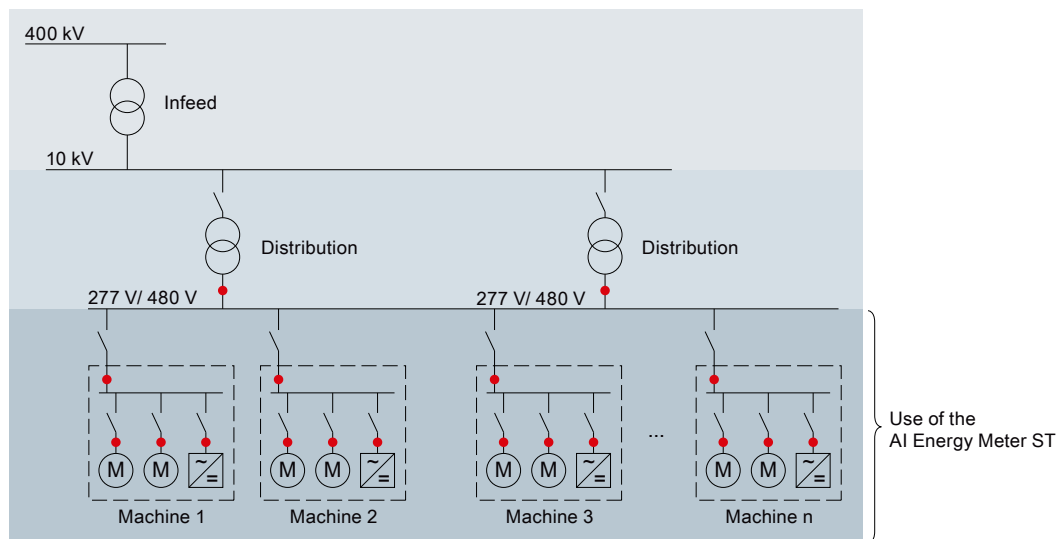
Figure 2-11 Use of the AI Energy Meter 480VAC ST
