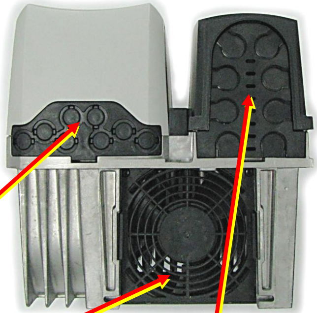
(11) Heatsink Cooling Fan PN: 3251-2038-00 Replacement Instructions CTRI243
