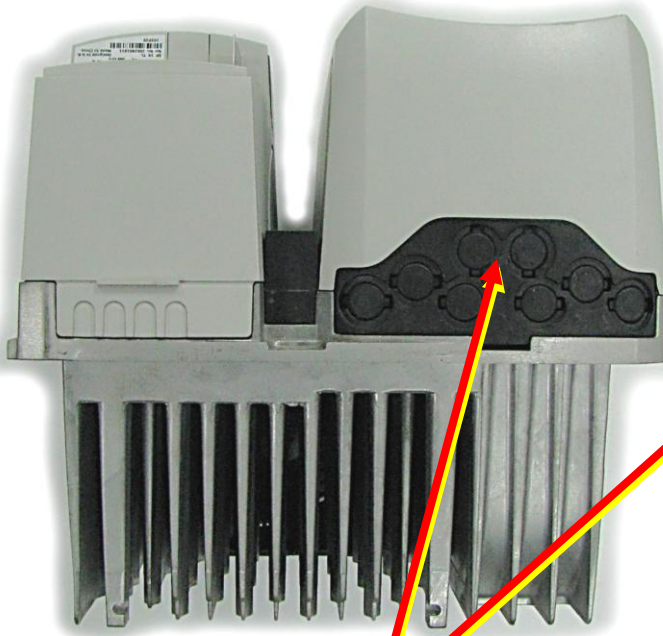
(10) Power Gland Plates PN: 3871-0050-04
