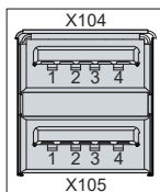
Fig. 6: USB output pin numbering
