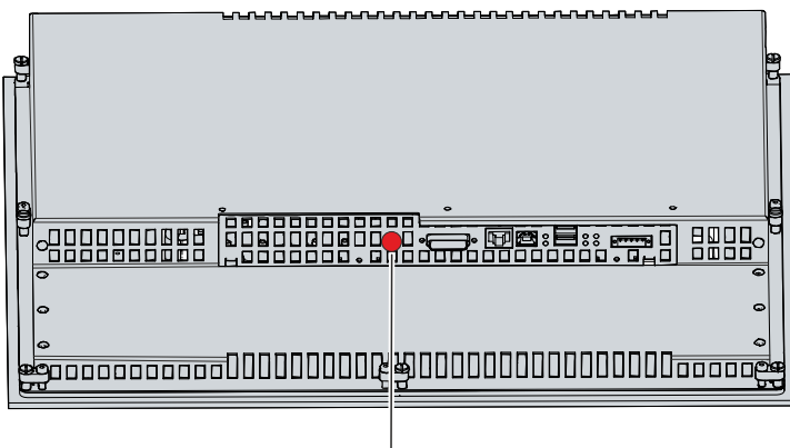
Fig. 15: Grounding bolt for functional earthing
