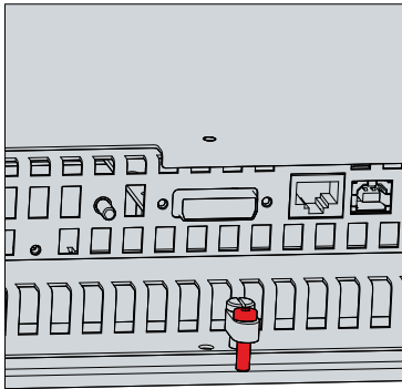
Fig. 16: Removal from the control cabinet
