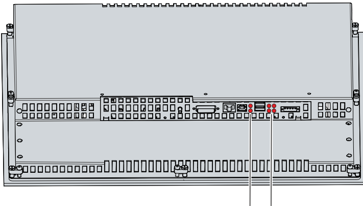
Fig. 8: Status LEDs
