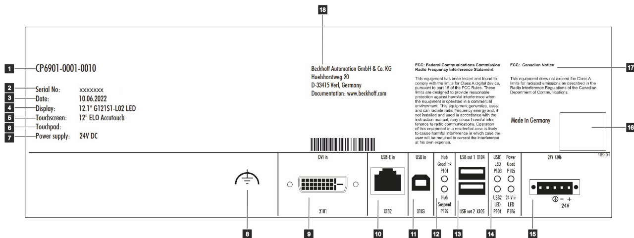
Fig. 9: Name plate
