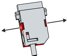
Fig. 14: Disassembly of the strain relief housing
