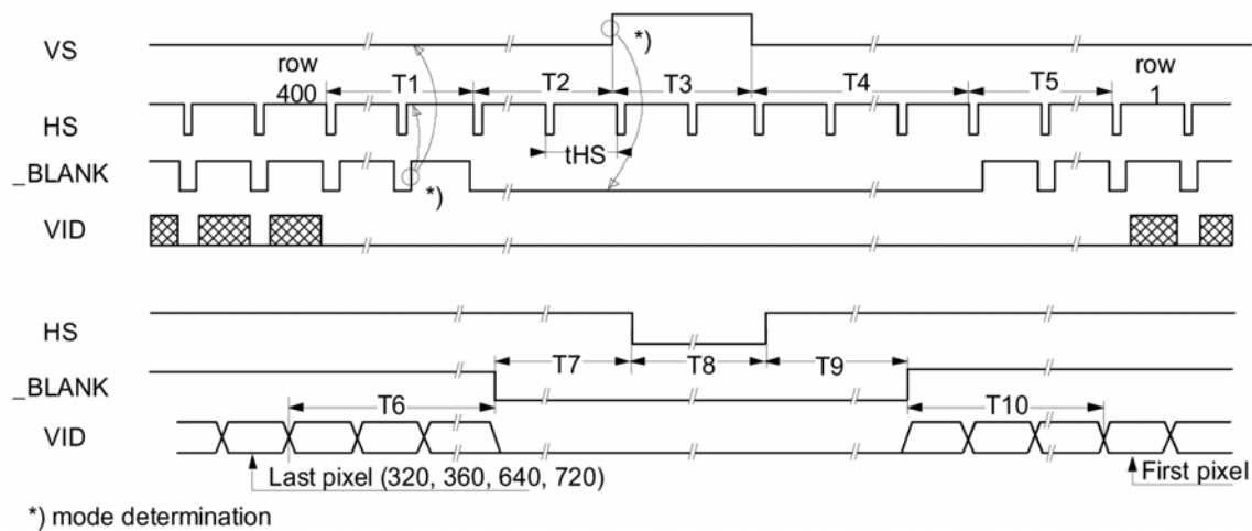
Figure 4. 400 Row VGA Modes (see page 9).
