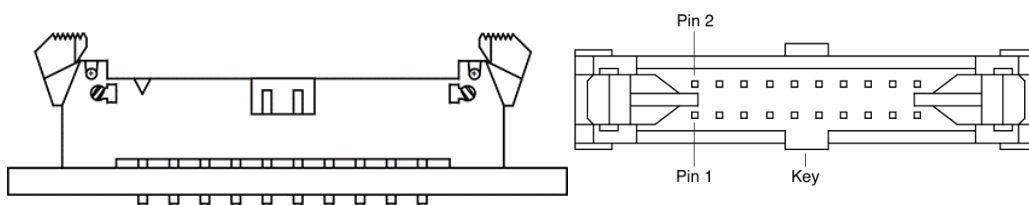
Figure 1. Locking data and power connector
