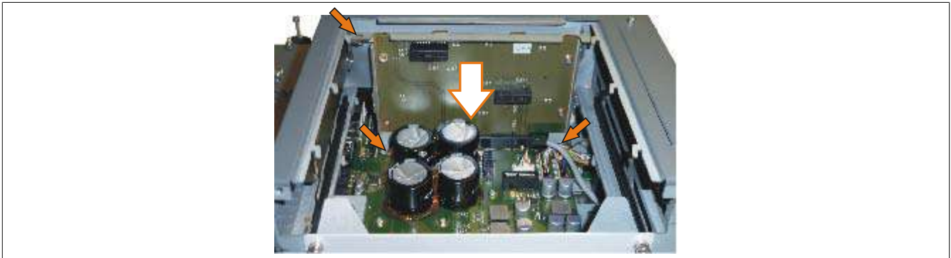
Figure 186: Installing the bus unit
