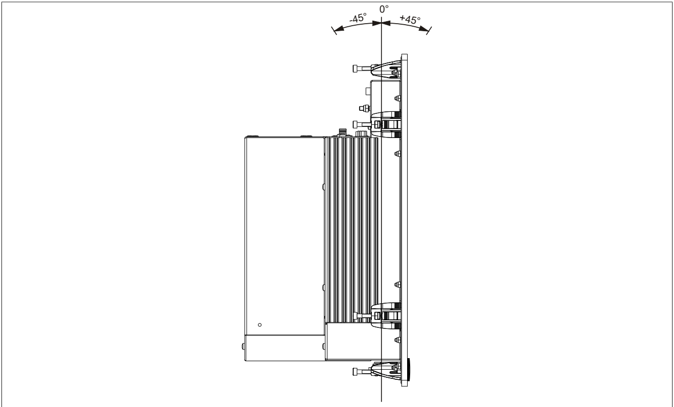
Figure 63: Mounting orientation 0° and +/- 45°
