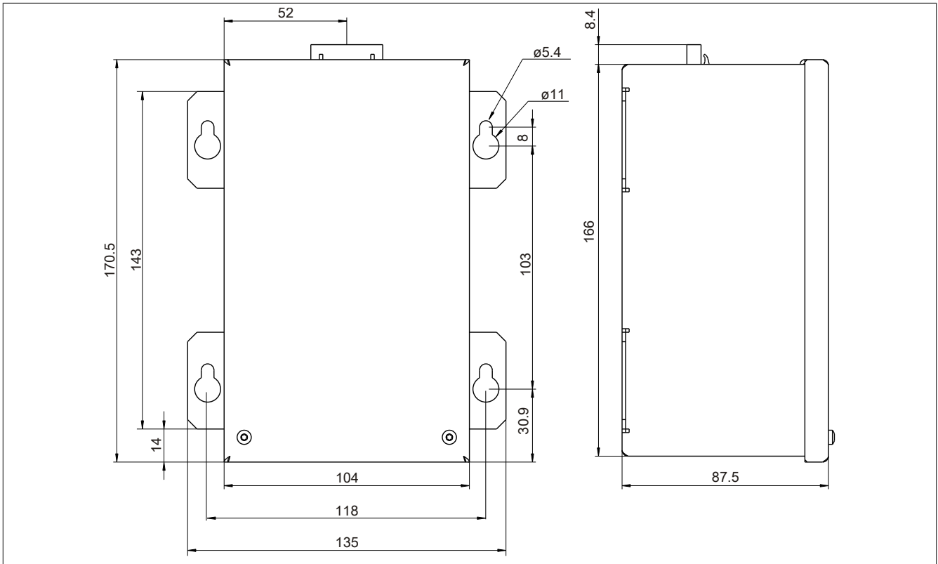
Figure 137: 5PC600.UPSB-00 - Dimensions
