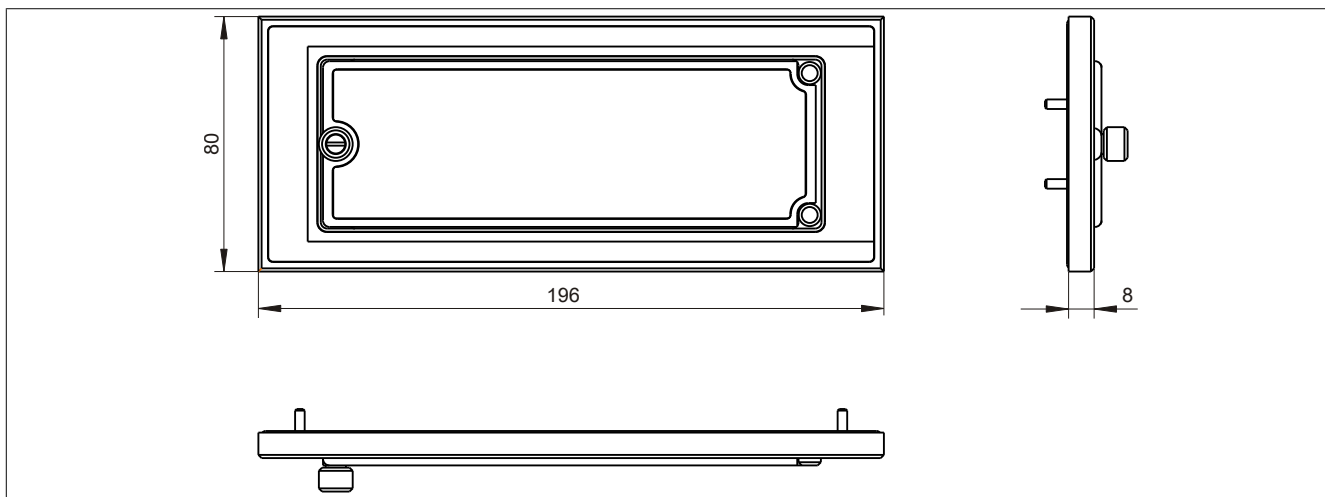
Figure 157: 5A5003.03 - Dimensions
