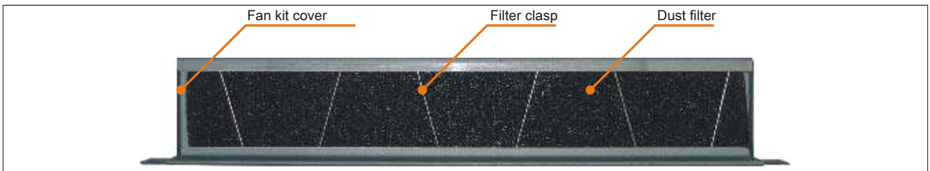
Figure 175: Securing the dust filter with the filter clasp
