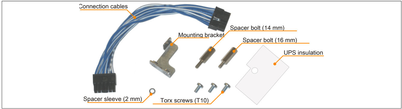
Figure 135: 5AC600. UPSI-00 Add-on UPS module - Installation materials
