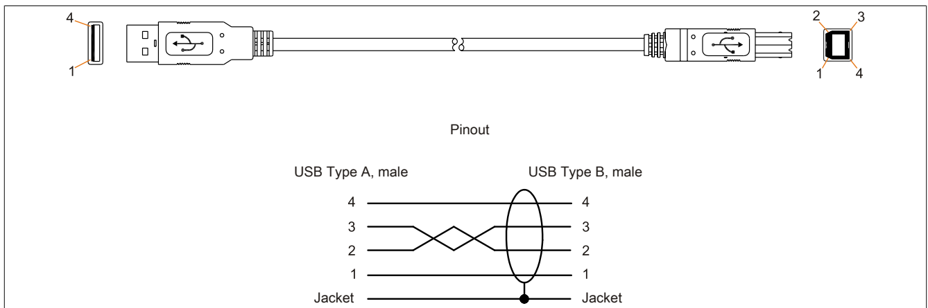
Figure 160: 5CAUSB.00xx-00 USB cables - Pinout
