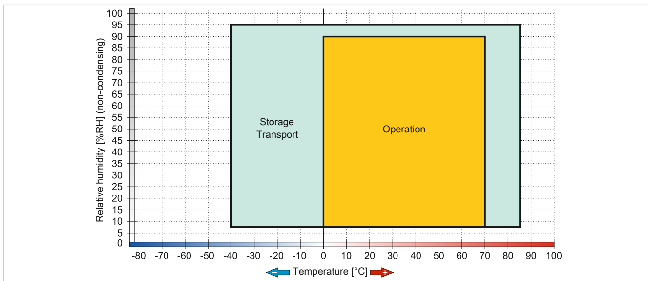
Figure 38: 5AC801.SSDI-03 ≤ Rev. C0 - Temperature/Humidity diagram
