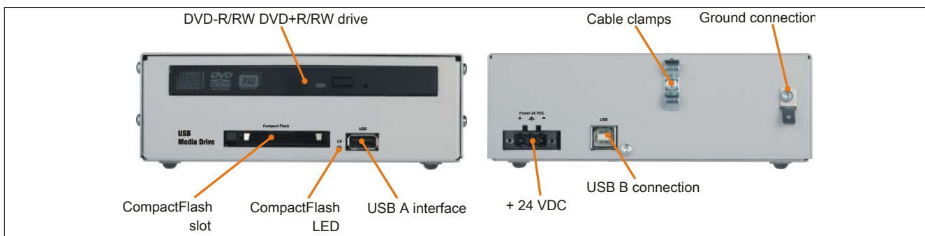
Figure 152: 5MD900.USB2-02 - Interfaces
