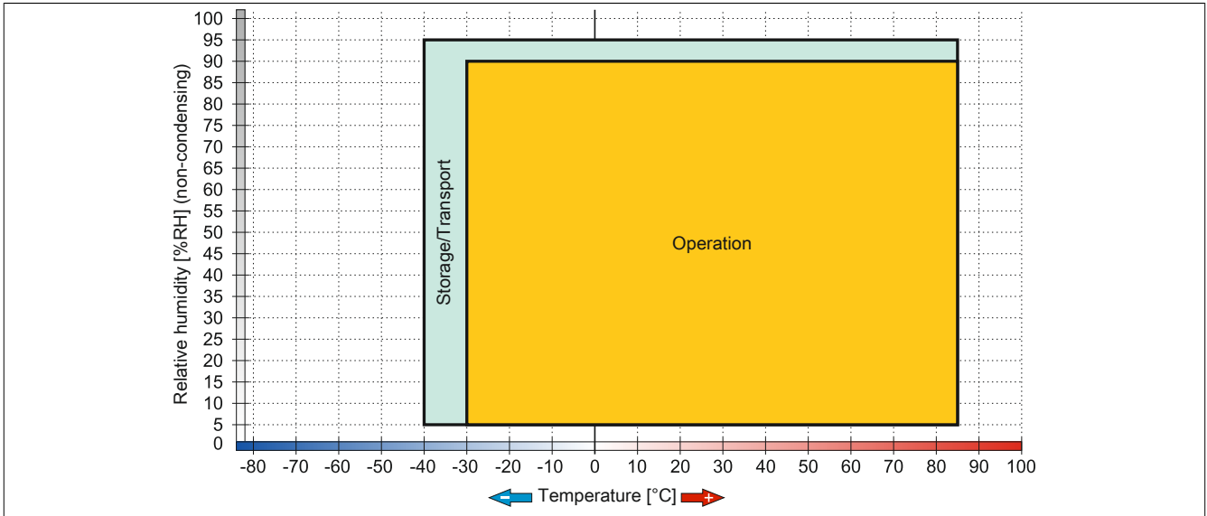
Figure 41: 5AC801.SSDI-04 ≥ Rev. D0 - Temperature/Humidity diagram
