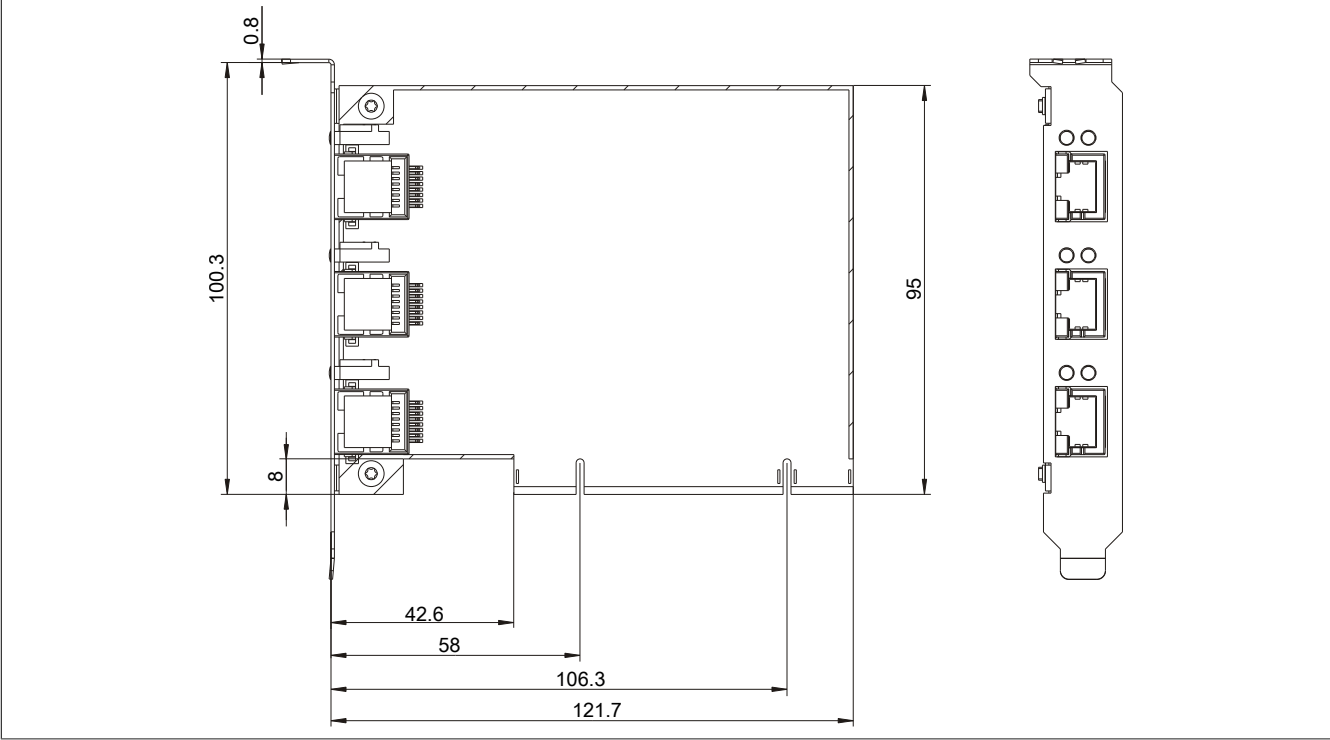
Figure 143: 5ACPCI.ETH3-01 - Dimensions
