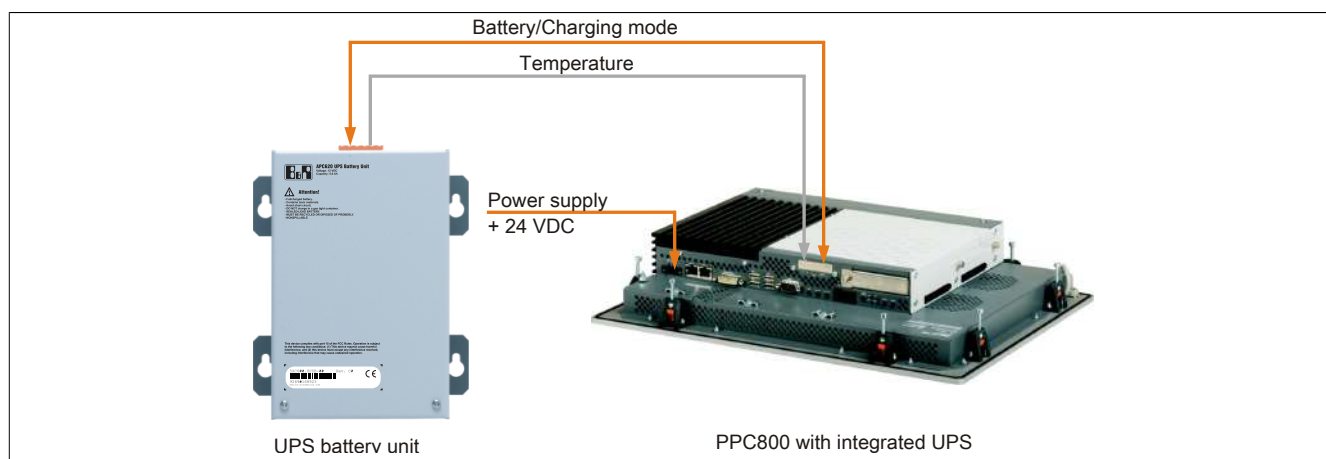
Figure 134: UPS principle
