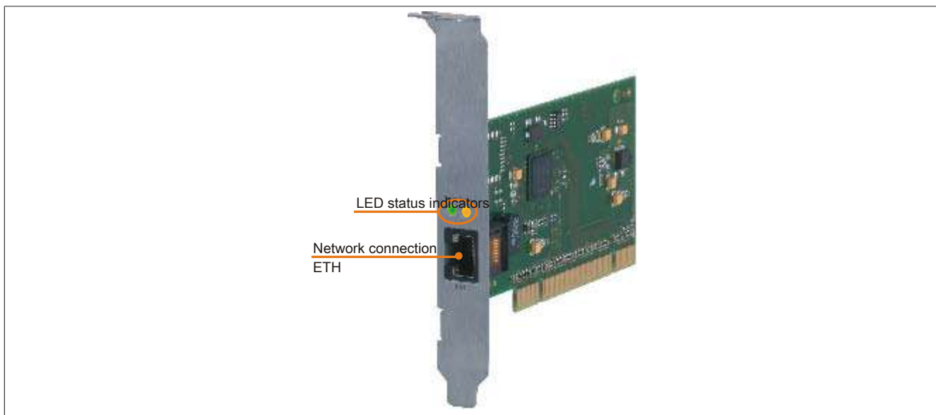
Figure 140: 5ACPCI.ETH1-01 - PCI 10/100 Ethernet card
