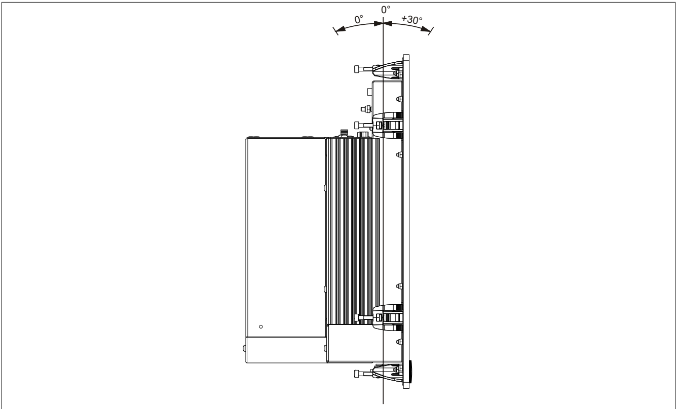
Figure 65: Mounting orientation with 5AC801.DVDS-00
