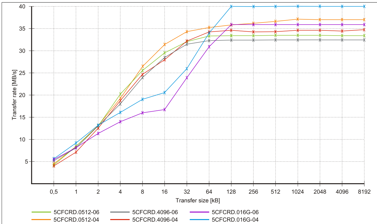
Figure 146: ATTO Disk Benchmark v2.34 read comparison - 5CFCRD.xxxx-04 and 5CFCRD.xxxx-06
