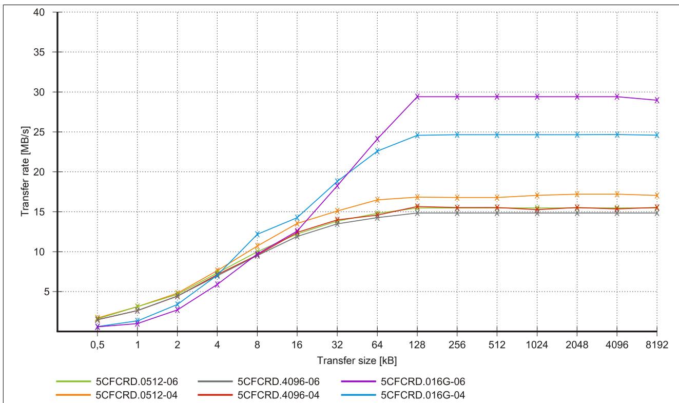
Figure 147: ATTO Disk Benchmark v2.34 write comparison - 5CFCRD.xxxx-04 and 5CFCRD.xxxx-06
