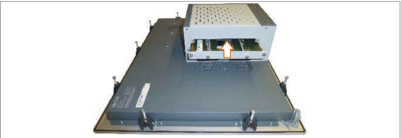
Figure 171: Installing the slide-in compact adapter
