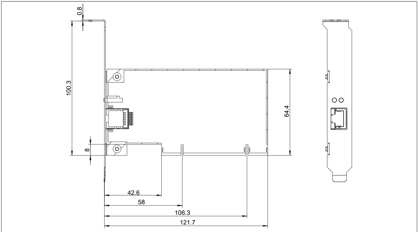
Figure 151: 5ACPCI.ETH1-01 - Dimensions
