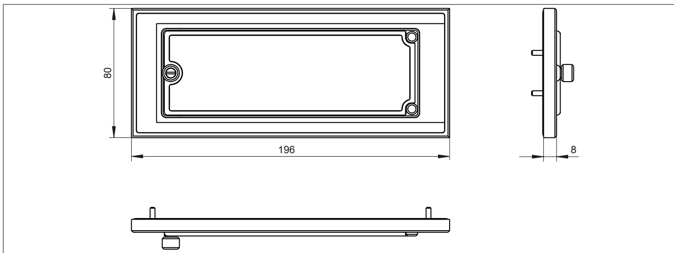
Figure 171: 5A5003.03 - Dimensions
