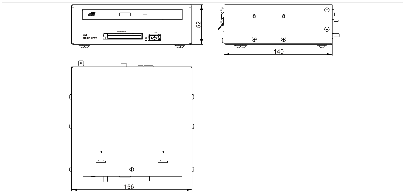
Figure 167: 5MD900.USB2-02 - Dimensions
