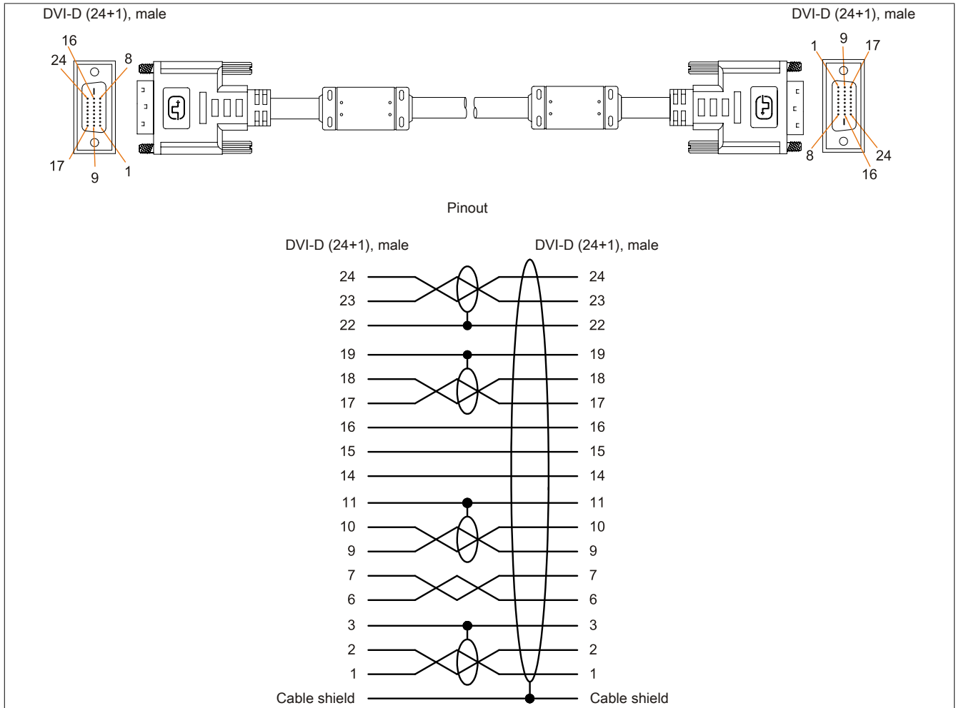
Figure 176: 5CADVI.0xxx-00 - Pinout
