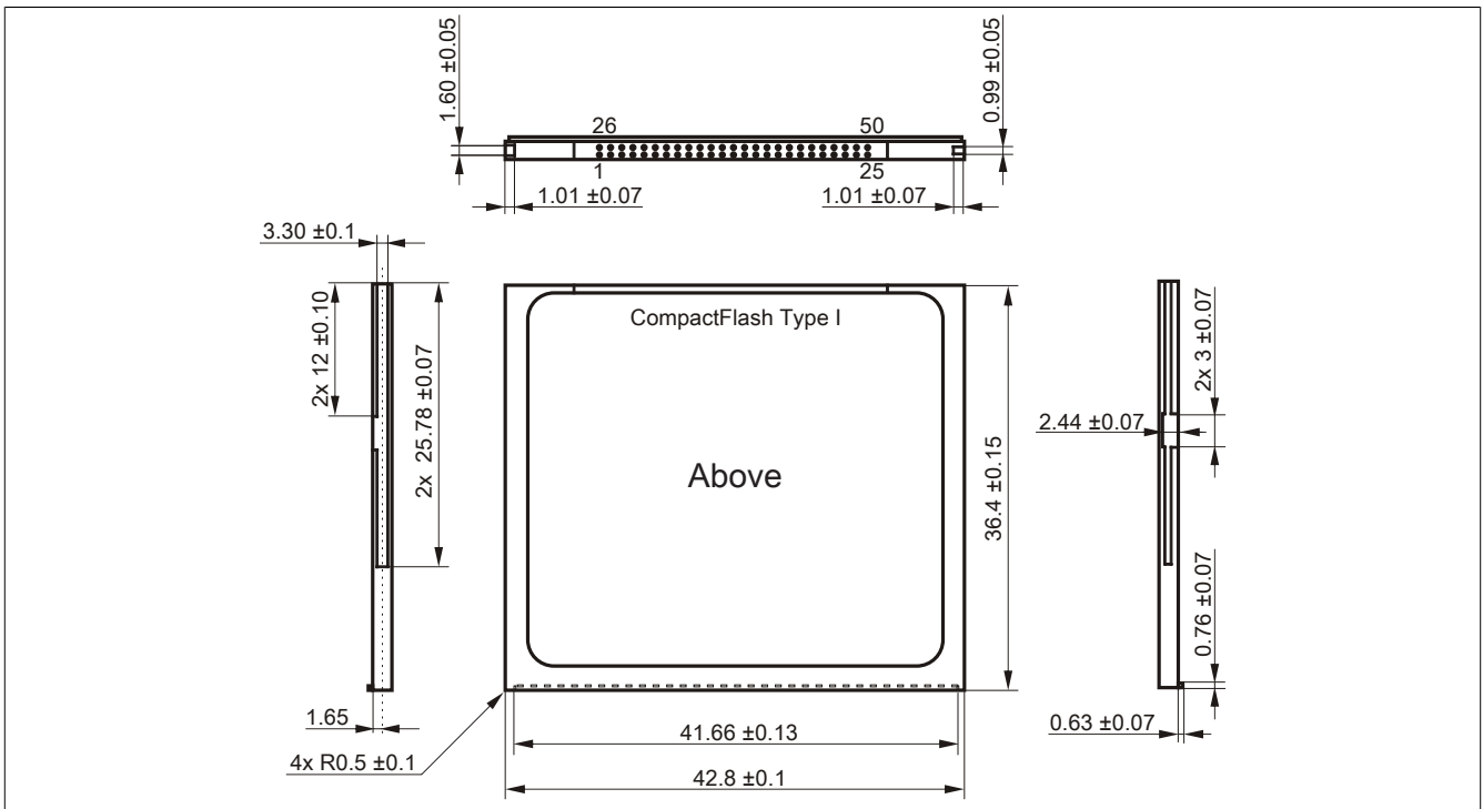
Figure 155: Type I CompactFlash card - Dimensions
