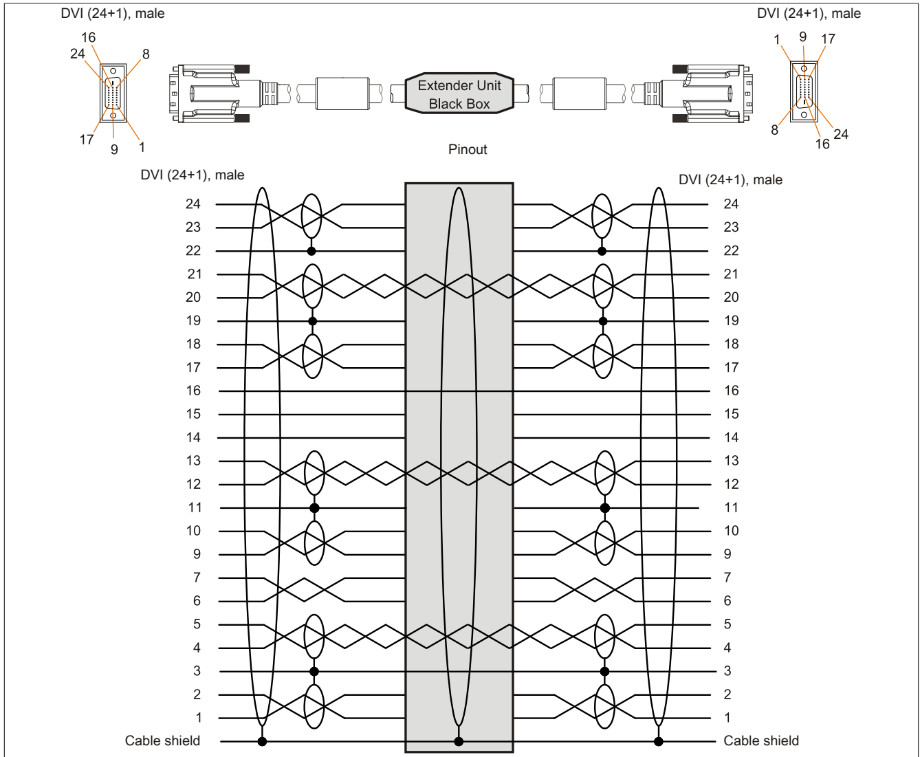
Figure 188: 5CASDL.0xx0-13 - Pinout
