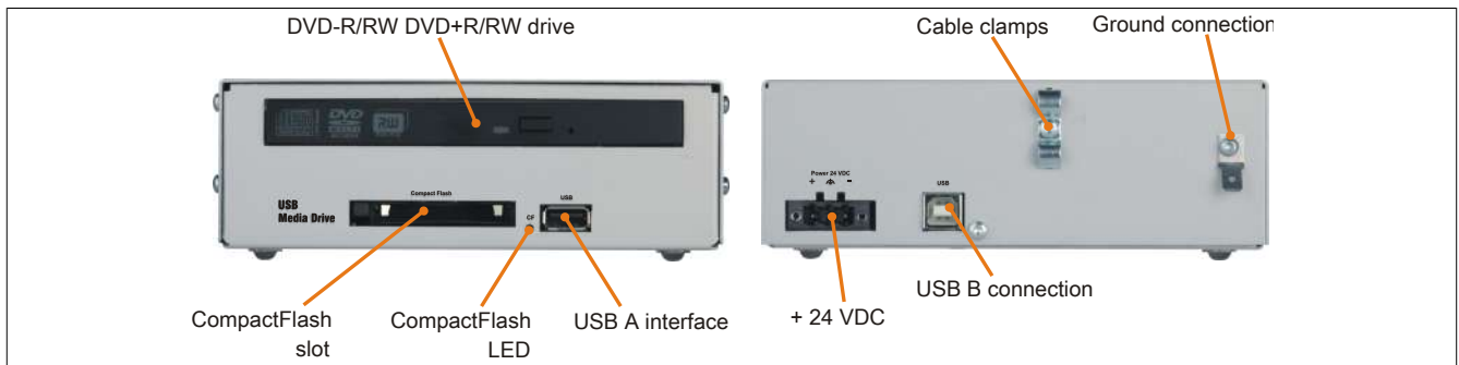
Figure 166: 5MD900.USB2-02 - Interfaces
