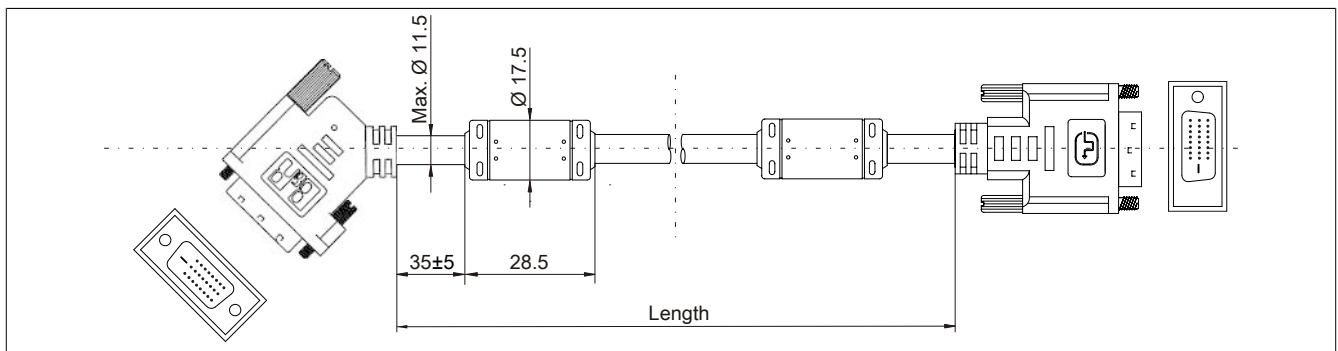
Figure 181: 5CASDL.0xxx-01 - Dimensions
