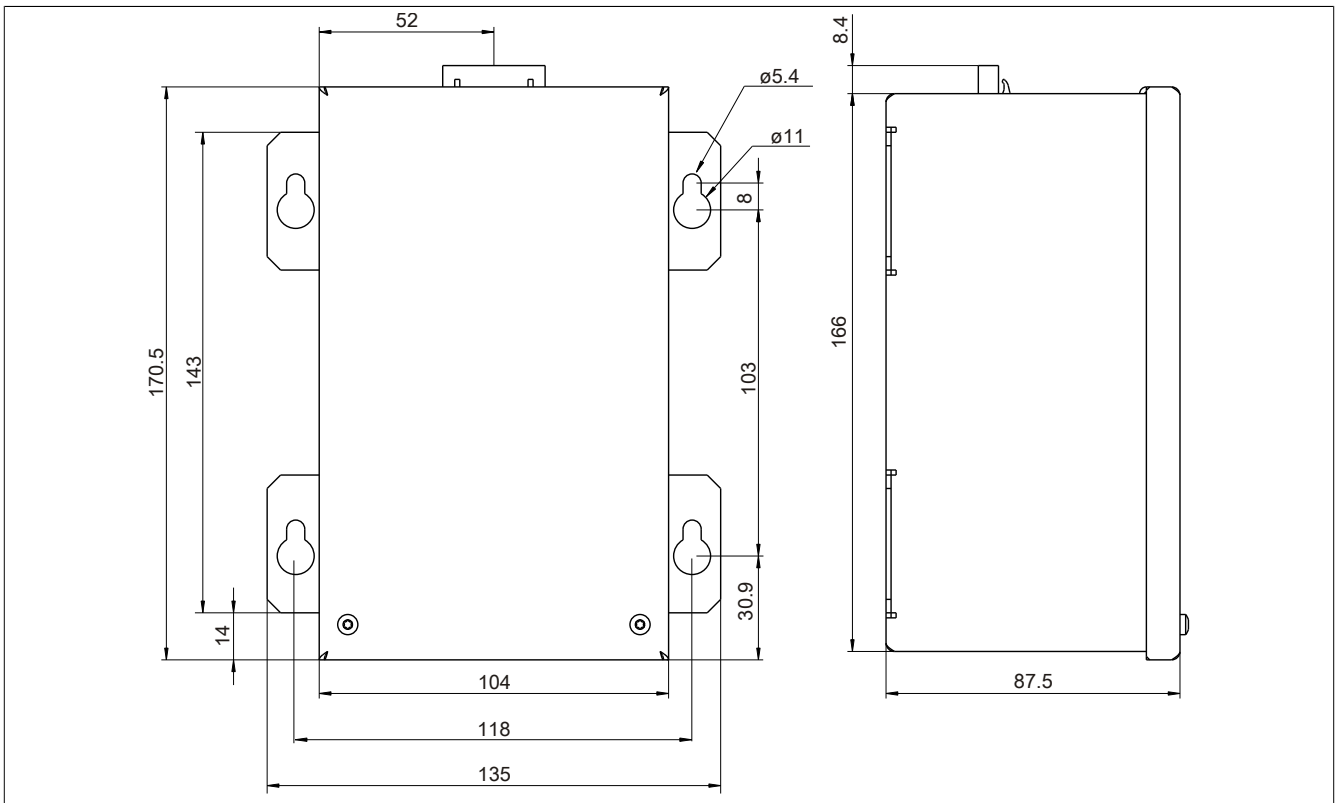
Figure 147: 5PC600.UPSB-00 - Dimensions
