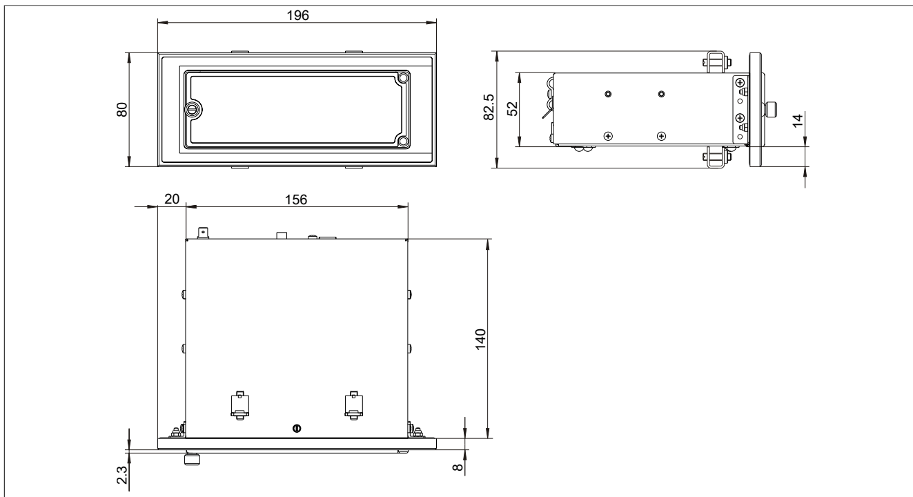
Figure 168: USB media drive with front cover - Dimensions
