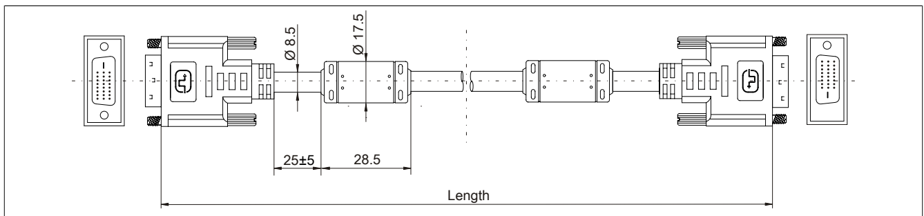
Figure 175: 5CADVI.0xxx-00 - Dimensions
