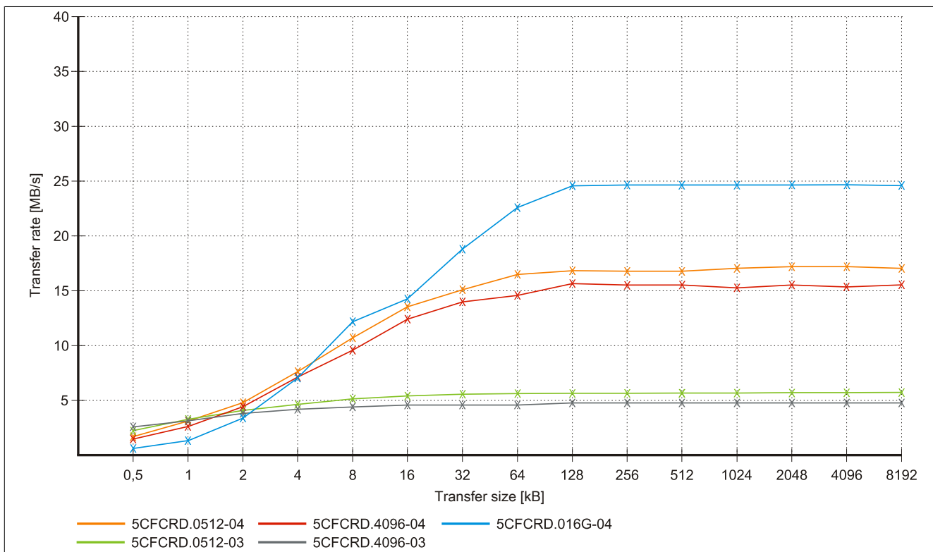
Figure 161: ATTO Disk Benchmark v2.34 write comparison - 5CFCRD.xxxx-03 and 5CFCRD.xxxx-04
