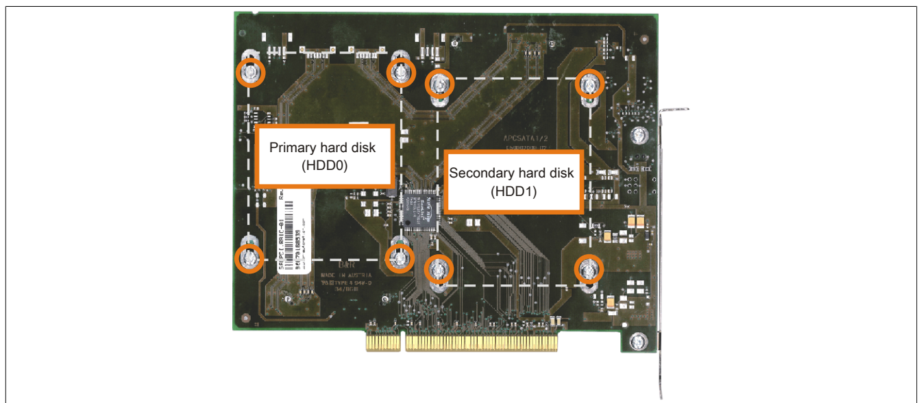
Figure 224: Screw layout on the back side of the 5ACPCI.RAIC-03 SATA RAID controller
