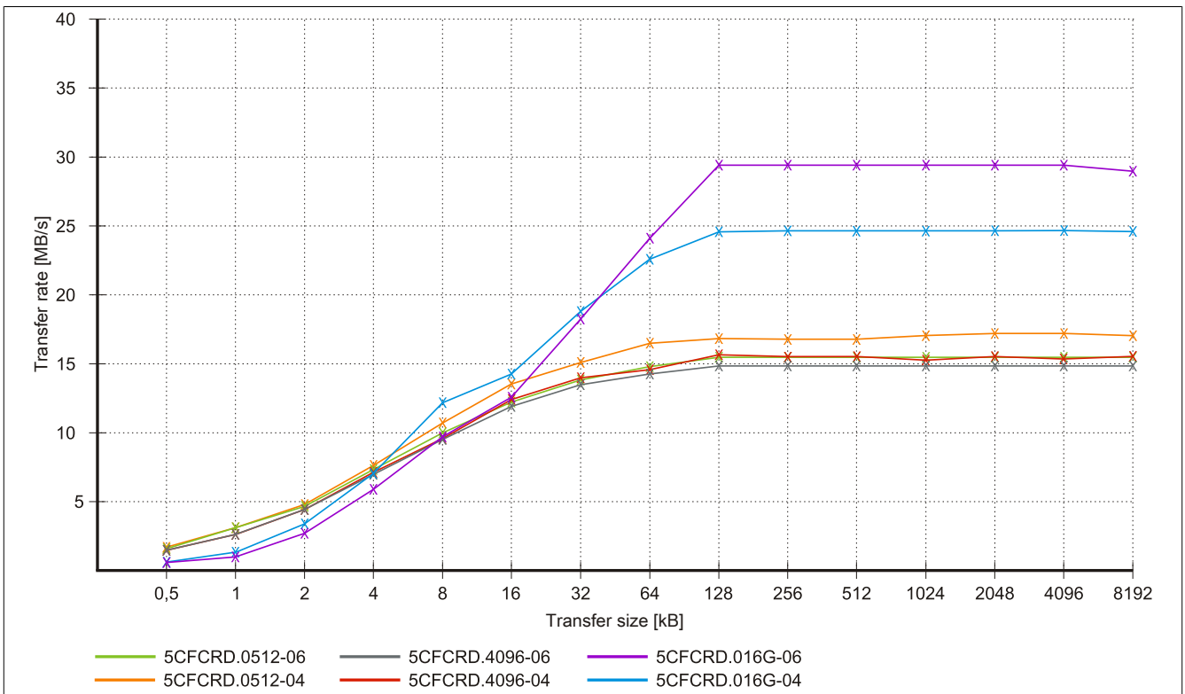
Figure 157: ATTO Disk Benchmark v2.34 write comparison - 5CFCRD.xxxx-04 and 5CFCRD.xxxx-06
