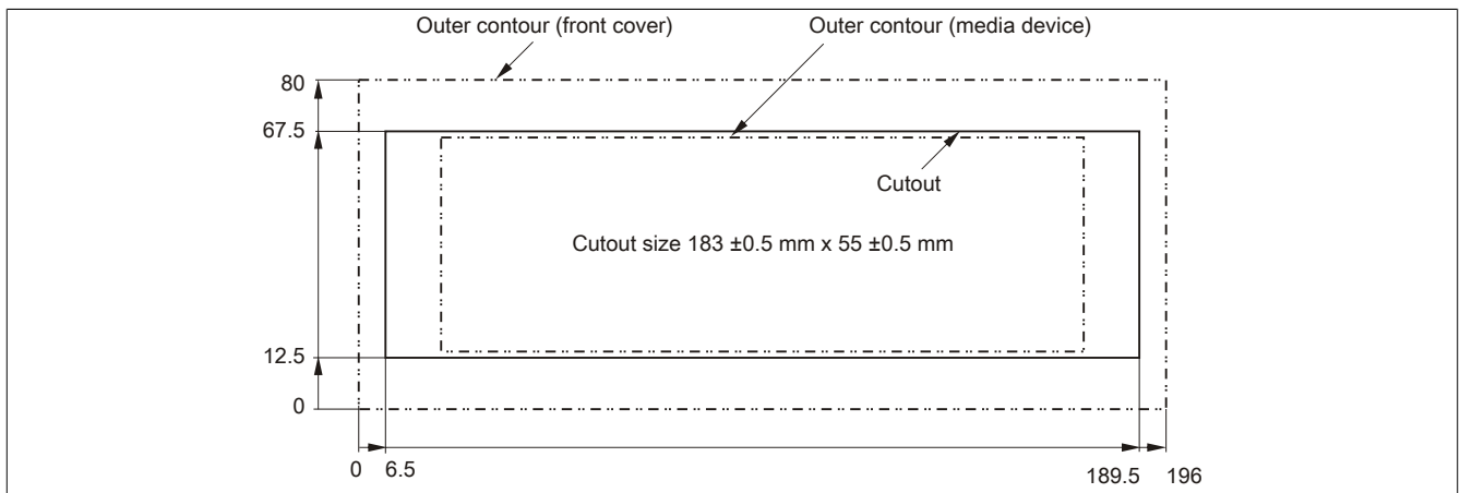
Figure 173: USB media drive with front cover - Installation cutout
