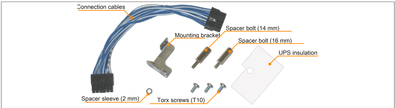
Figure 206: 5AC600.UPI-00 Add-on UPS module - Installation materials
