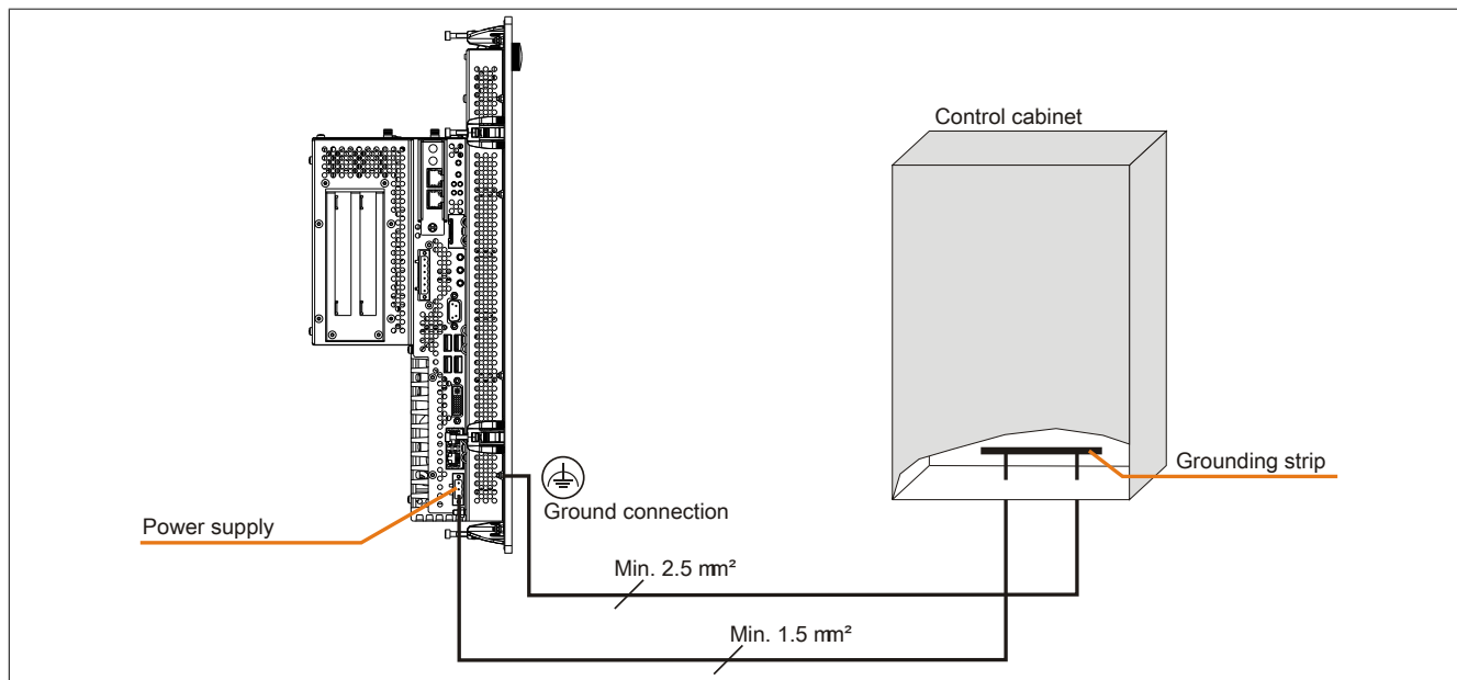
Figure 72: Grounding concept
