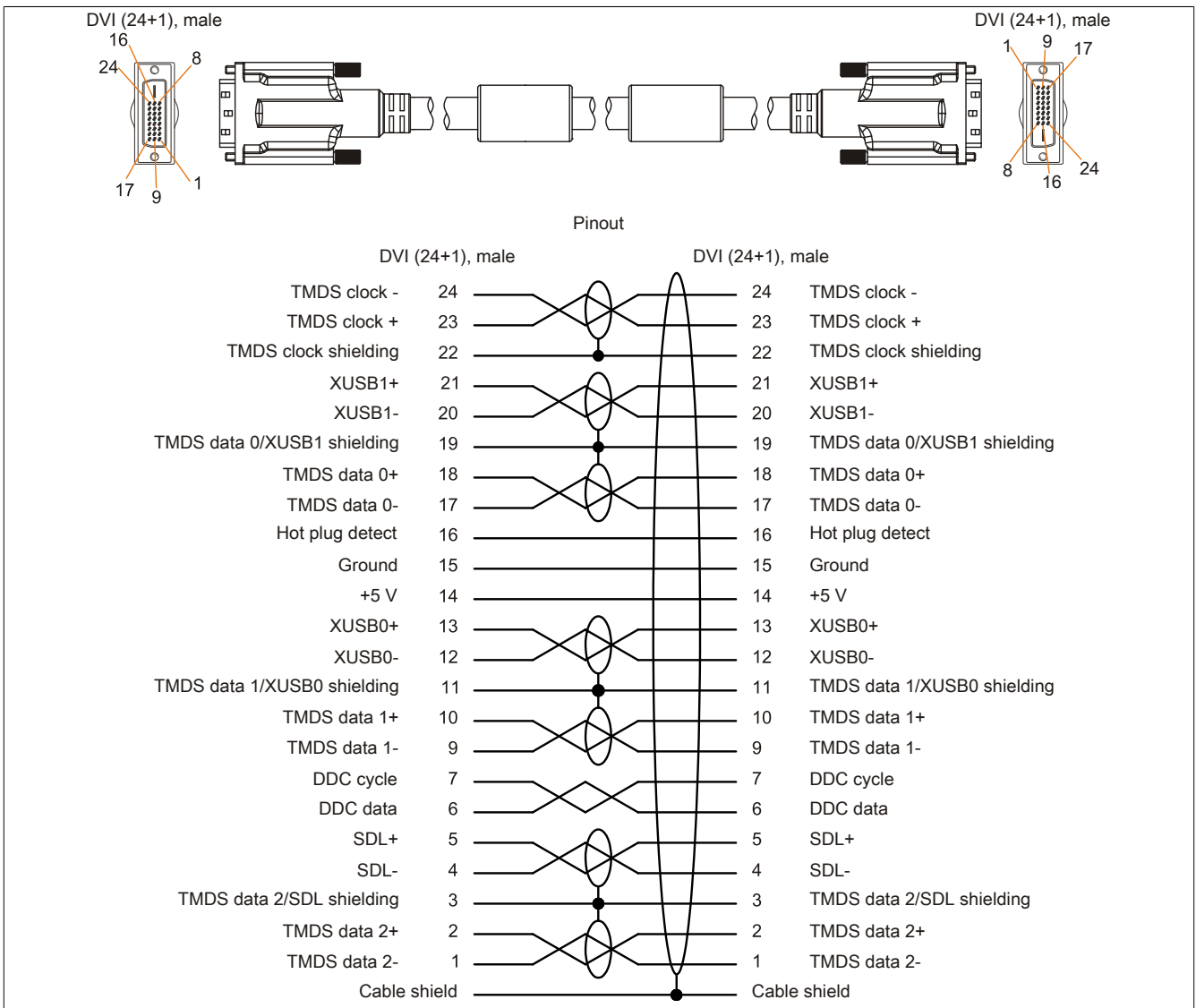
Figure 185: 5CASDL.0xxx-03 - Pinout
