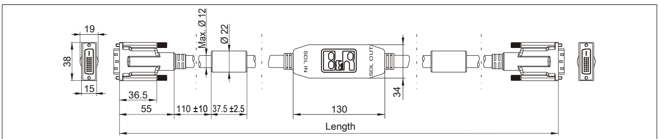
Figure 187: 5CASDL.0xx0-13 - Dimensions
