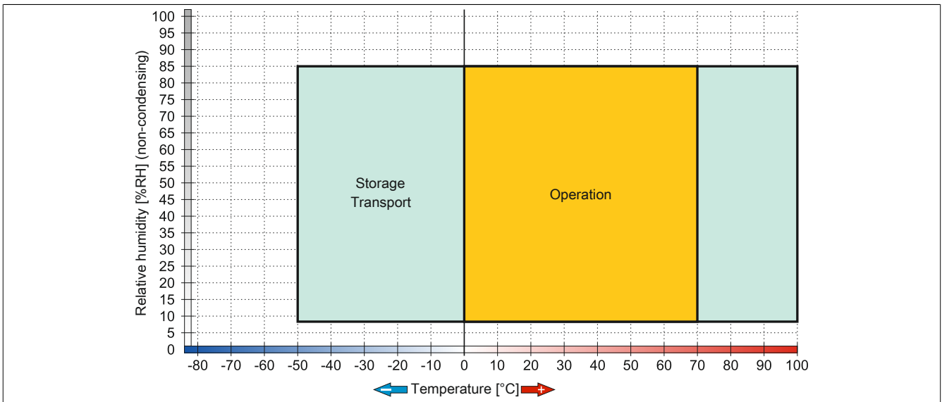
Figure 154: 5CFCRD.xxxx-06 - Temperature/Humidity diagram for CompactFlash cards
