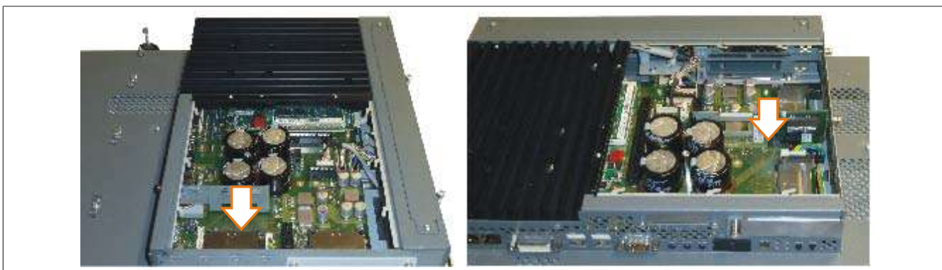
Figure 218: Installing the 5AC803.BC01-00 adapter
