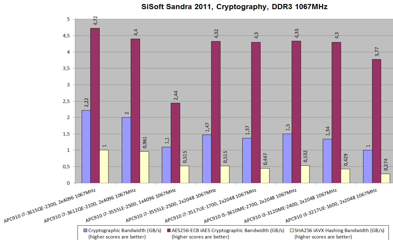
Figure 34: Results for SiSoft Sandra 2011, Cryptography, DDR3 1067MHz – APC910/PPC900
