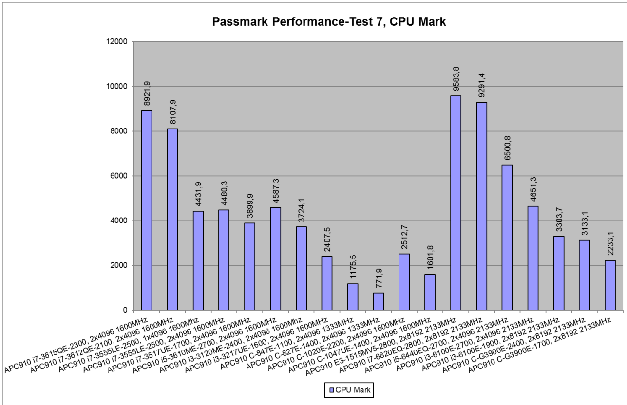
Figure 89: Results for Passmark Performance Test 7.0, CPU Mark – APC910
