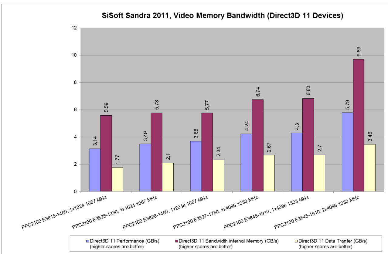
Figure 70: Results for SiSoft Sandra 2011, Video Memory Bandwidth (Direct3D 11 Devices) – APC2100/PPC2100
