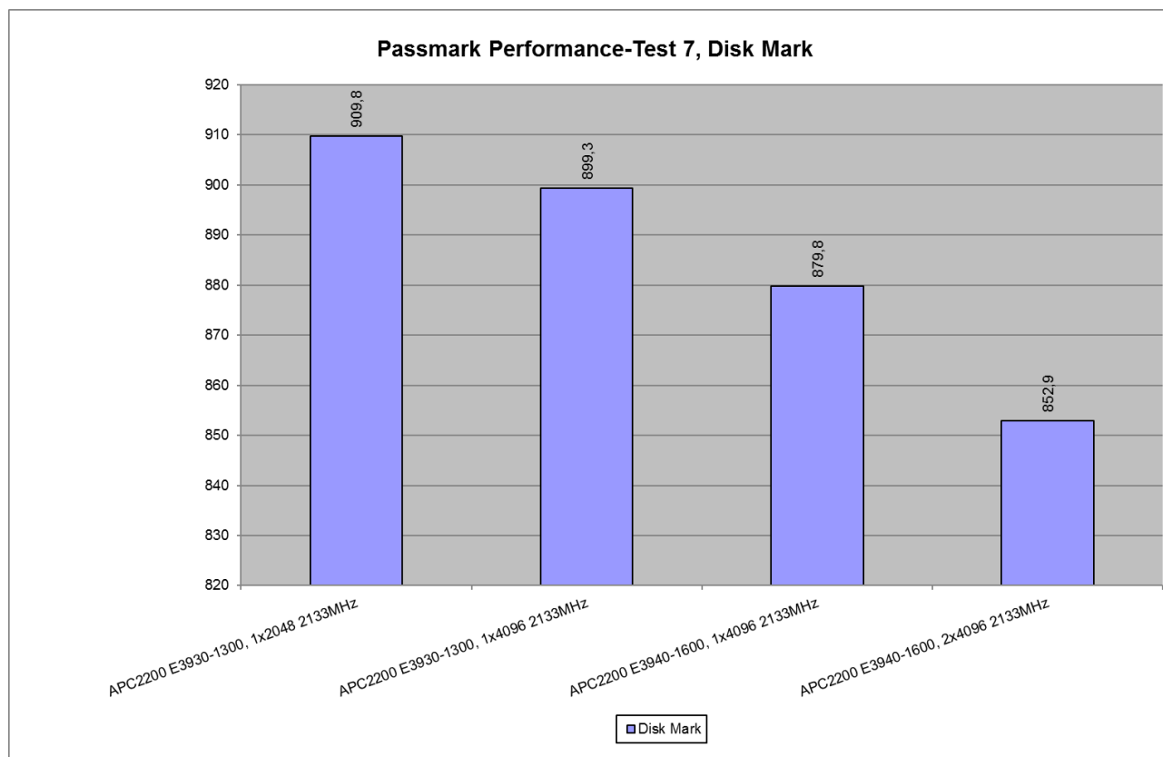
Figure 111: Results Passmark Performance Test 7.0, Disk Mark – APC2200/PPC2200
