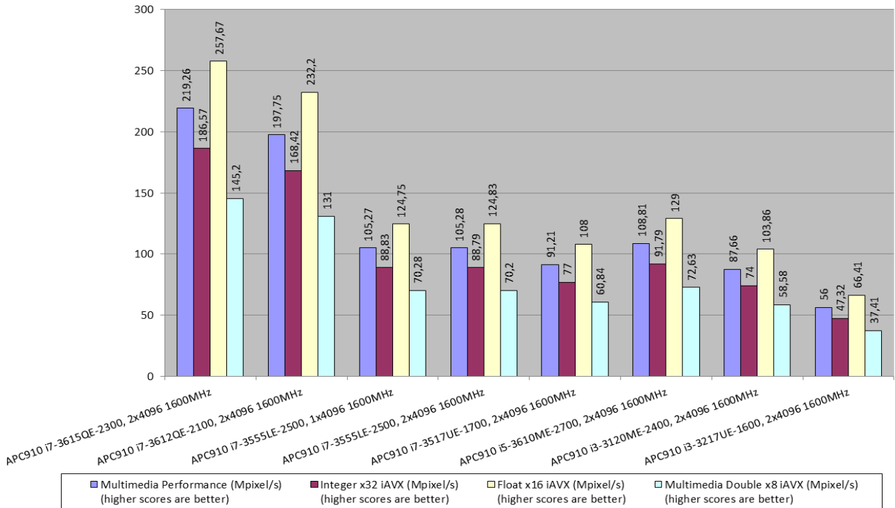
Figure 30: Results for SiSoft Sandra 2011, Processor Multi-Media (HM77 Chipset), DDR3 1600MHz – APC910/PPC900
