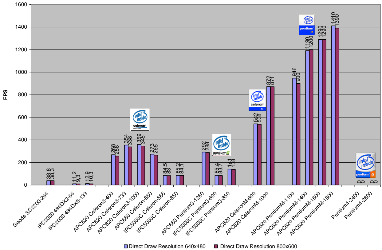
Figure 11 – Results for WinBench99 Direct Draw
