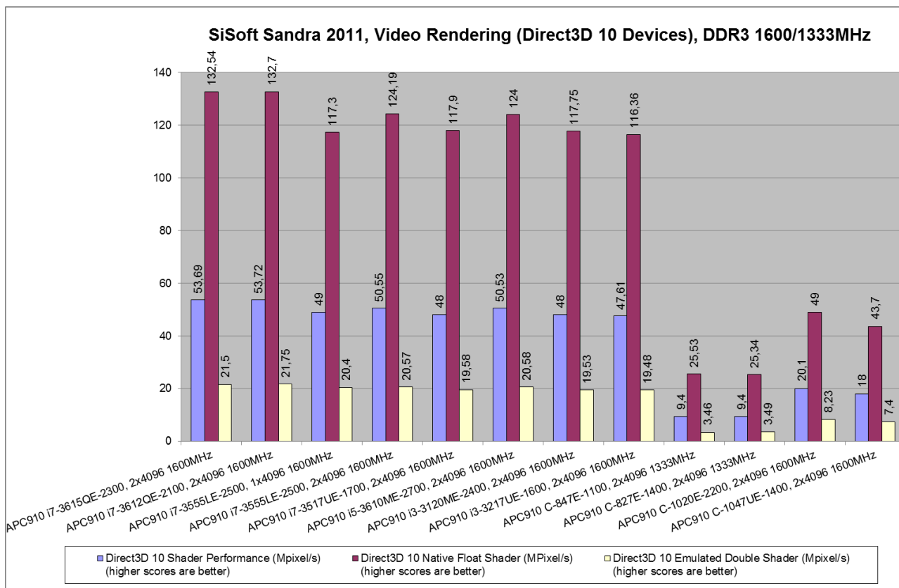
Figure 40: Results for SiSoft Sandra 2011, Video Rendering (Direct3D 10 Devices), DDR3 1600/1333MHz – APC910/PPC900
