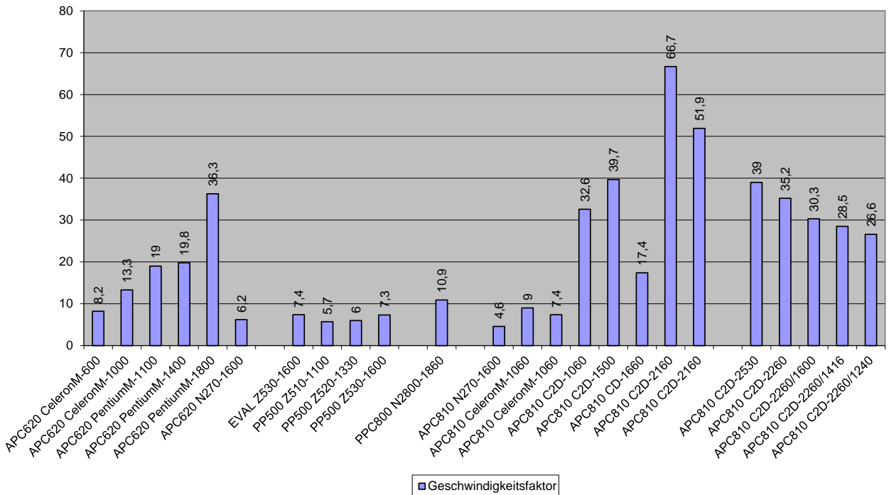
Figure 25 - Results for Sisoft Sandra Pro Business 2007, cache and memory bandwidth
