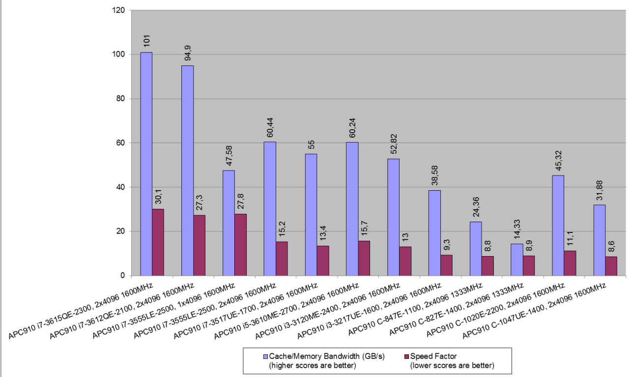
Figure 59: Results for SiSoft Sandra 2011, Cache and Memory, DDR3 1600/1333MHz – APC910/PPC900
