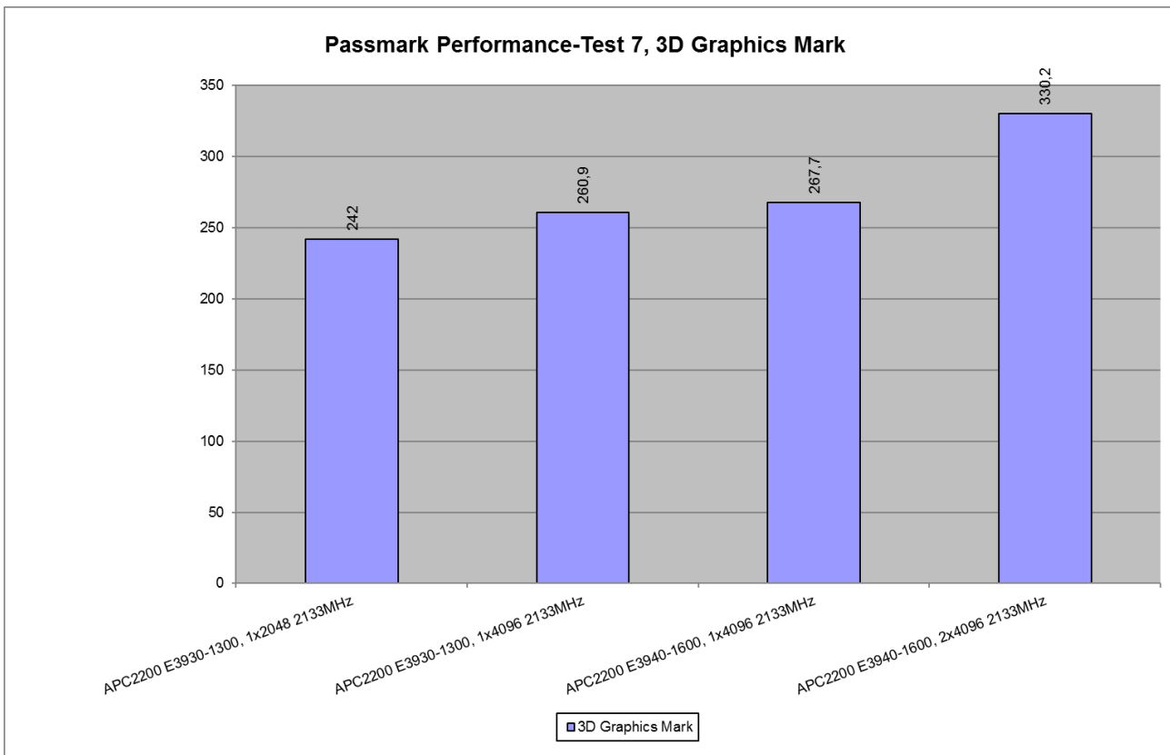
Figure 109: Results for Passmark Performance Test 7.0, 3D Graphics Mark – APC2200/PPC2200
