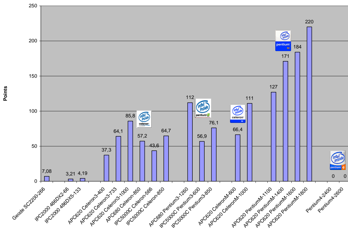
Figure 9 – Results for WinBench99 CPUMark99
