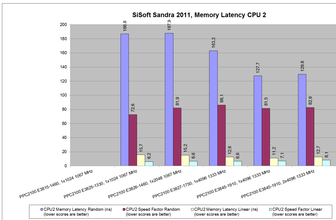
Figure 73: Results for SiSoft Sandra 2011, Memory Latency CPU2 – APC2100/PPC2100
