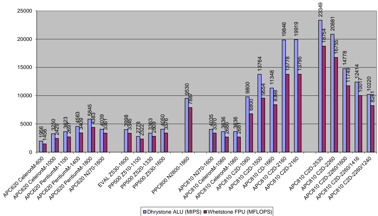
Figure 21 - Results for Sisoft Sandra Pro Business 2007 CPU Arithmetic
