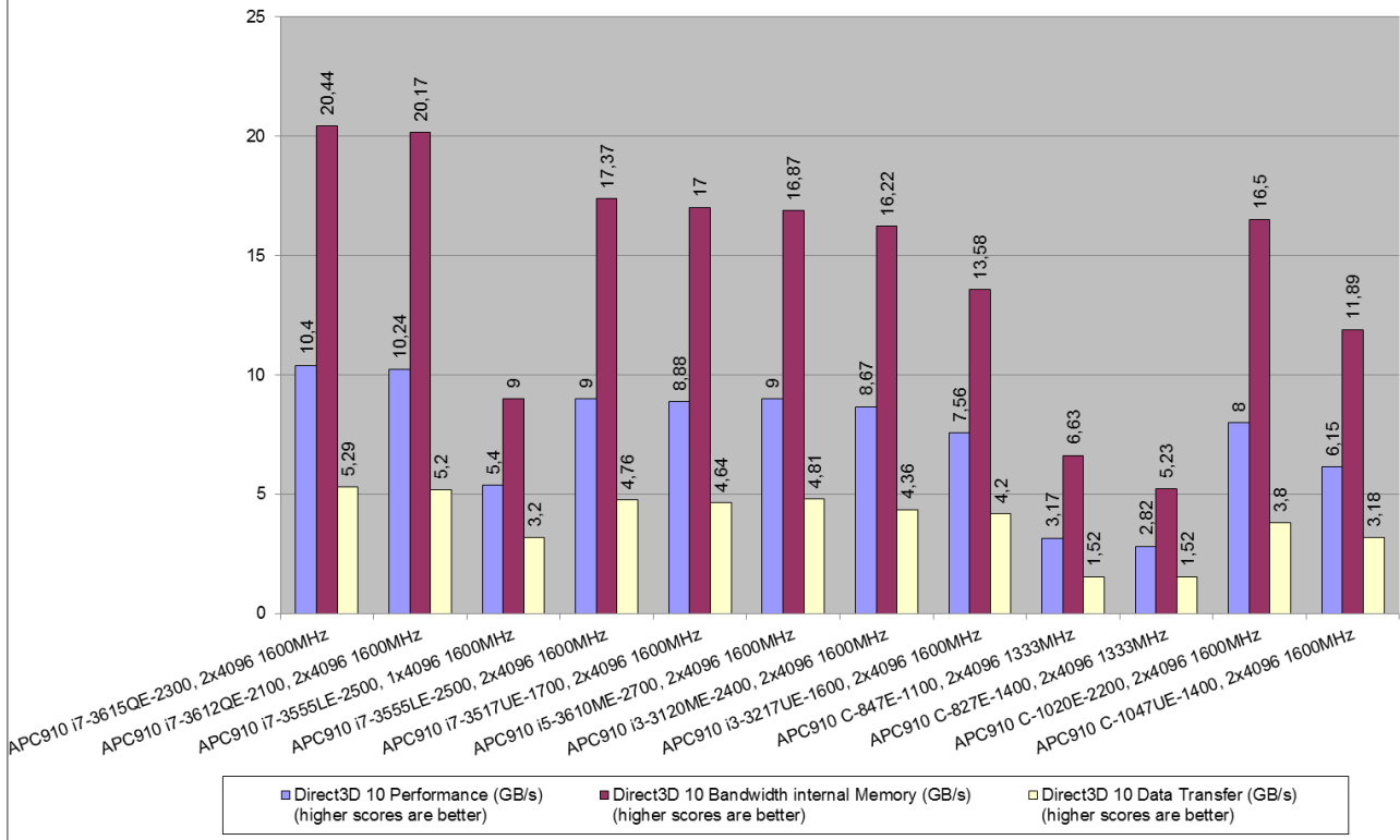
Figure 46: Results for SiSoft Sandra 2011, Video Memory Bandwidth (Direct3D 10 Devices), DDR3 1600/1333MHz – APC910/PPC900
