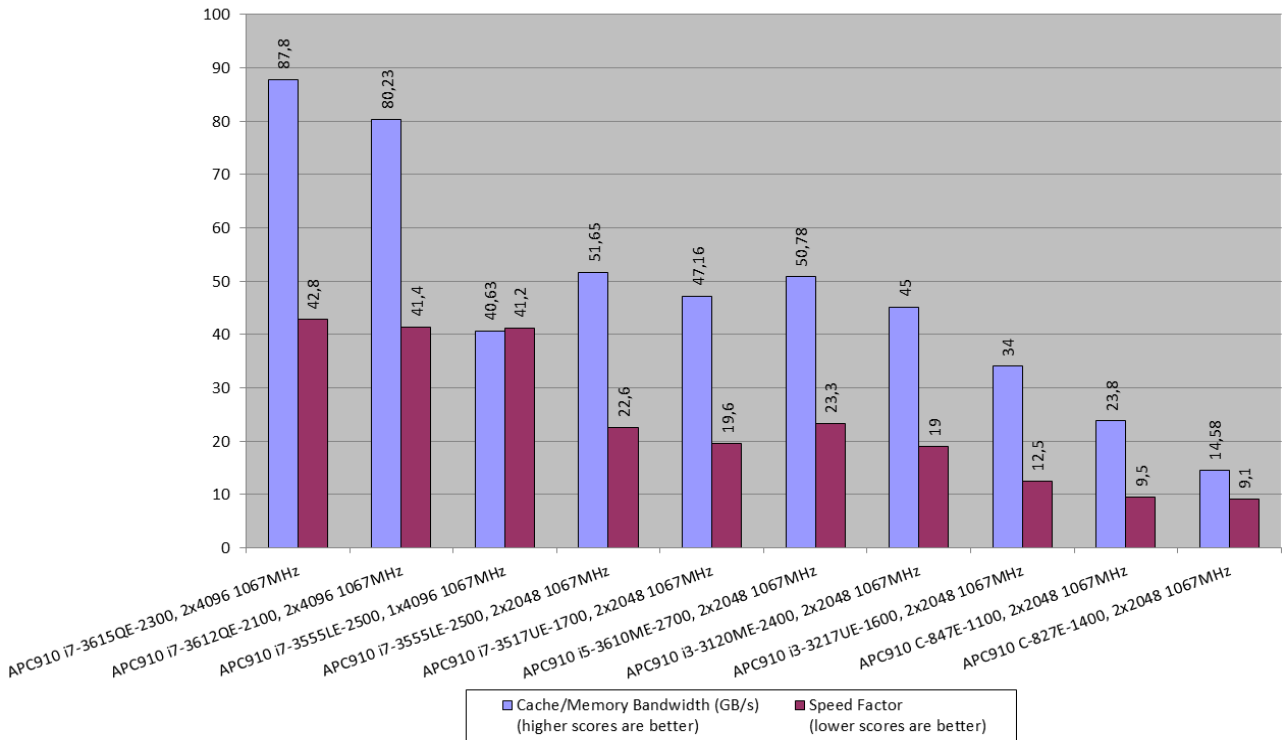
Figure 58: Results for SiSoft Sandra 2011, Cache and Memory, DDR3 1067MHz – APC910/PPC900
