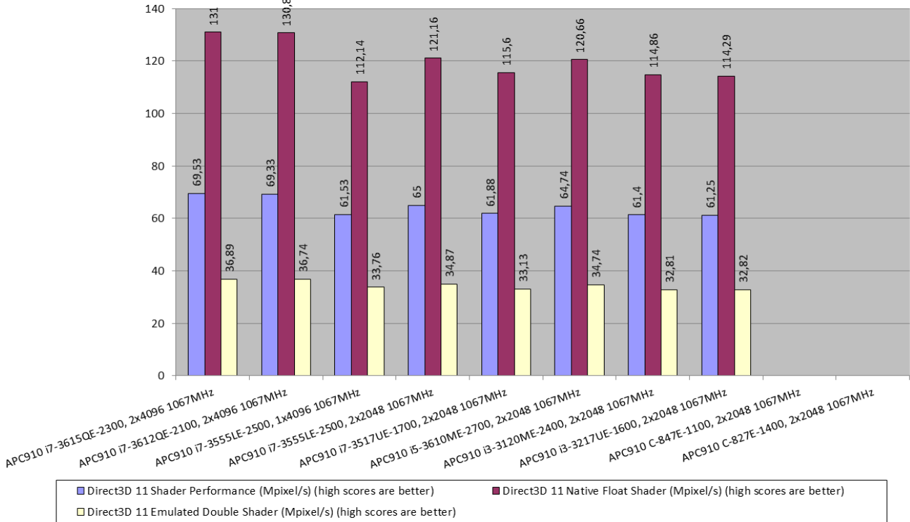
Figure 43: Results for SiSoft Sandra 2011, Video Rendering (Direct3D 11 Devices), DDR3 1067MHz – APC910/PPC900
