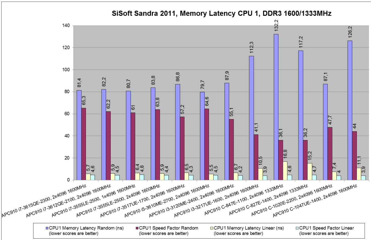
Figure 55: Results for SiSoft Sandra 2011, Memory Latency CPU1, DDR3 1600/1333MHz – APC910/PPC900
