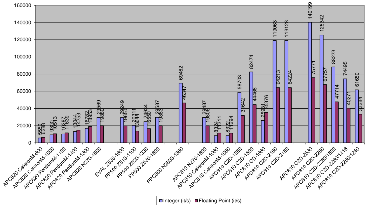
Figure 22 - Results for Sisoft Sandra Pro Business 2007, CPU MultiMedia
