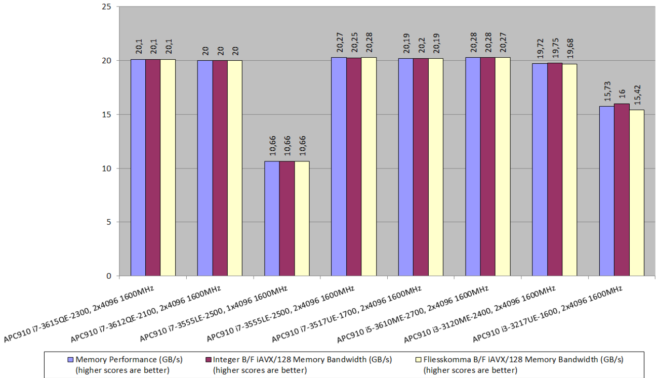
Figure 52: Results for SiSoft Sandra 2011, Memory Bandwidth (QM77 Chipset), DDR3 1600MHz – APC910/PPC900
