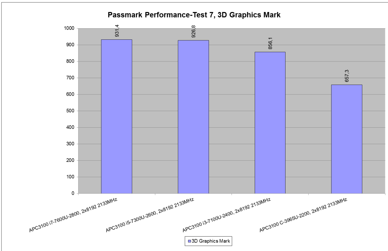
Figure 103: Results for Passmark Performance Test 7.0, 3D Graphics Mark – APC3100/PPC3100
