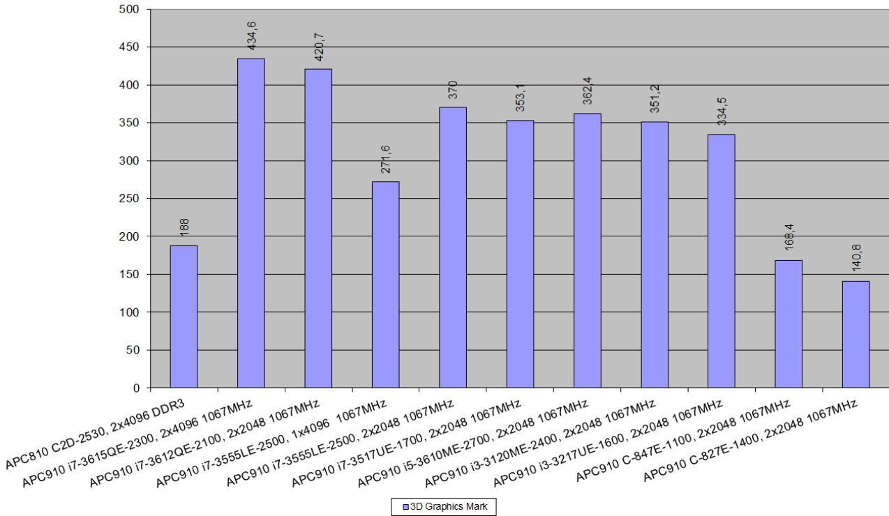
Figure 82: Results for Passmark Performance Test 7.0, 3D Graphics Mark, DDR3 1067MHz – APC910/PPC900
