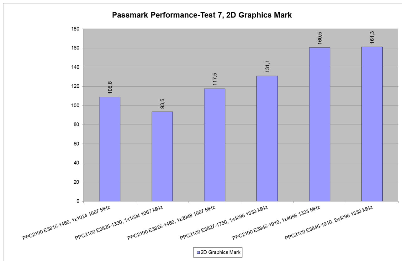
Figure 96: Results for Passmark Performance Test 7.0, 2D Graphics Mark – APC2100/PPC2100
