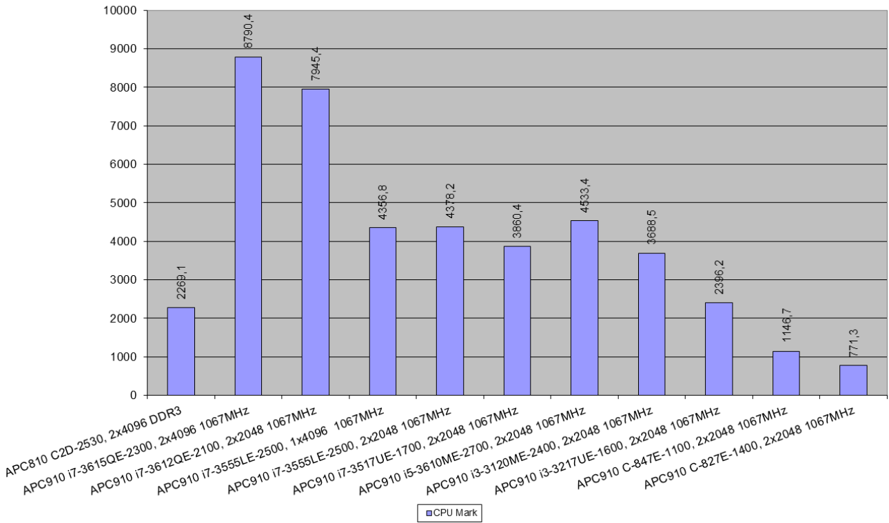
Figure 78: Results for Passmark Performance Test 7.0, CPU Mark, DDR3 1067MHz – APC910/PPC900
