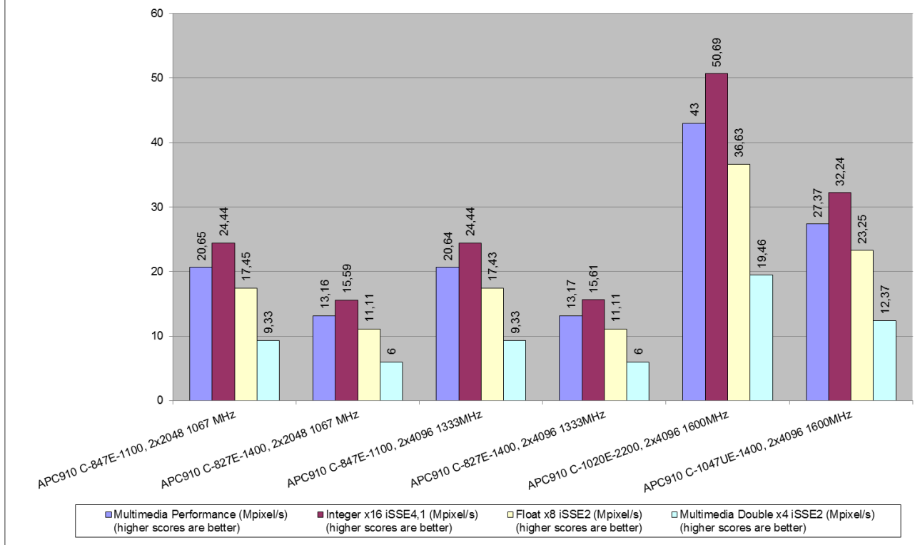
Figure 31: Results for SiSoft Sandra 2011, Processor Multi-Media (HM76 Chipset), DDR3 1067/1333/1600MHz – APC910/PPC900
