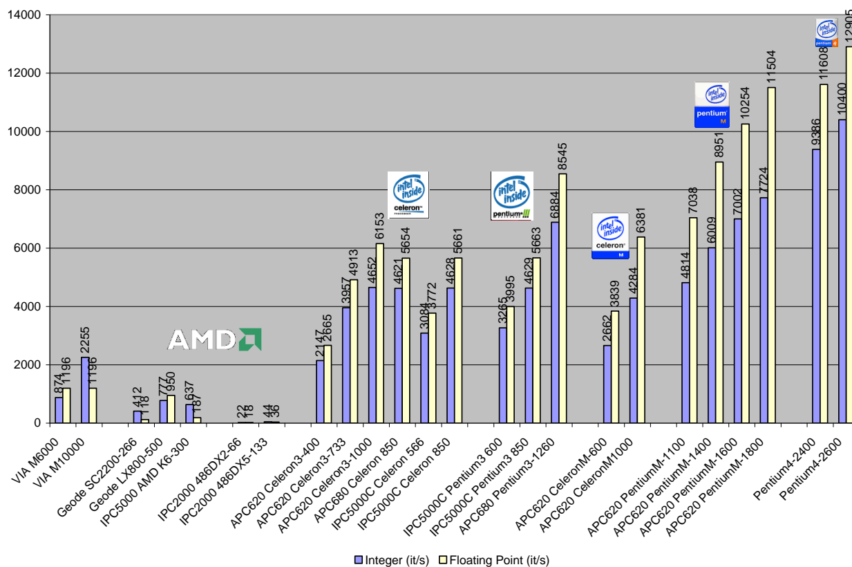
Figure 2 – Results for Siisoft Sandra 2002 Prof CPU multimedia
