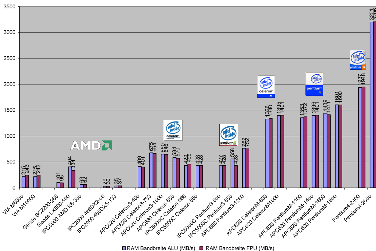
Figure 3 – Results for Siisoft Sandra 2002 Prof memory bandwidth
