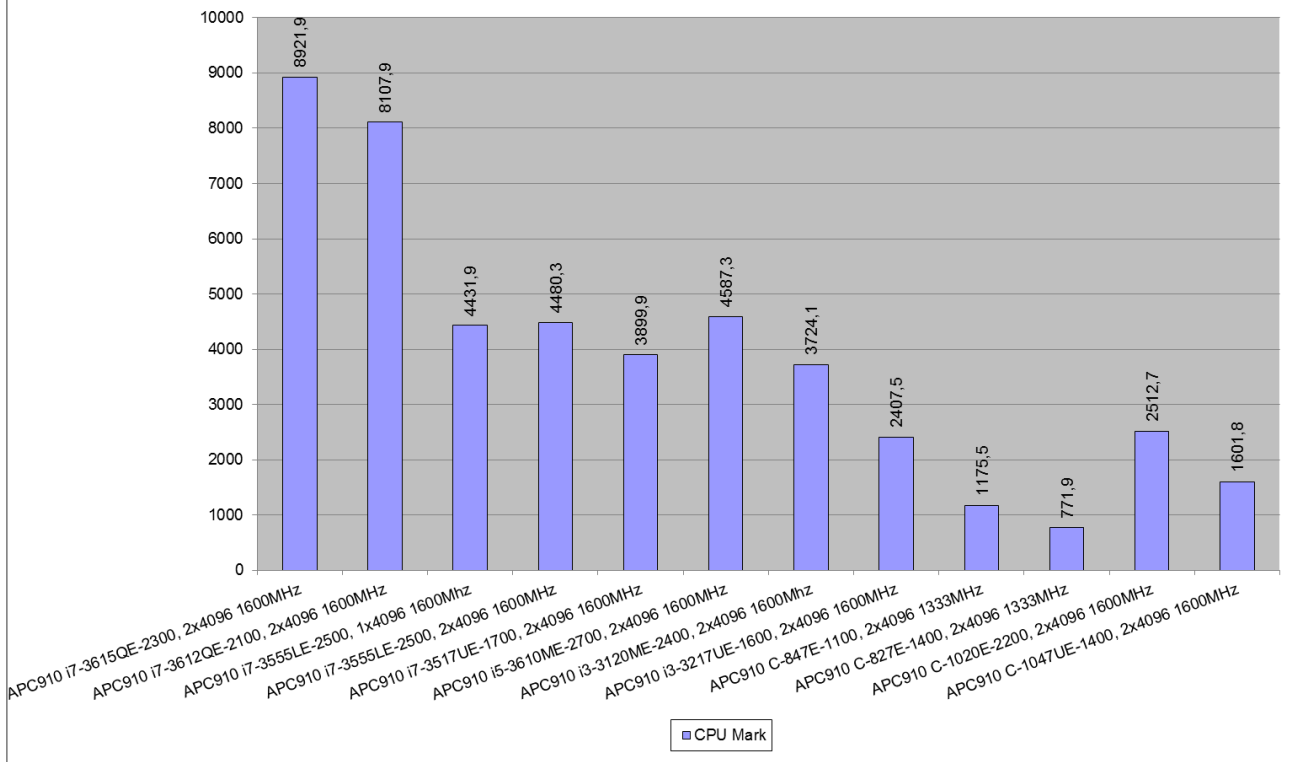
Figure 79: Results for Passmark Performance Test 7.0, CPU Mark, DDR3 1600/1333MHz – APC910/PPC900
