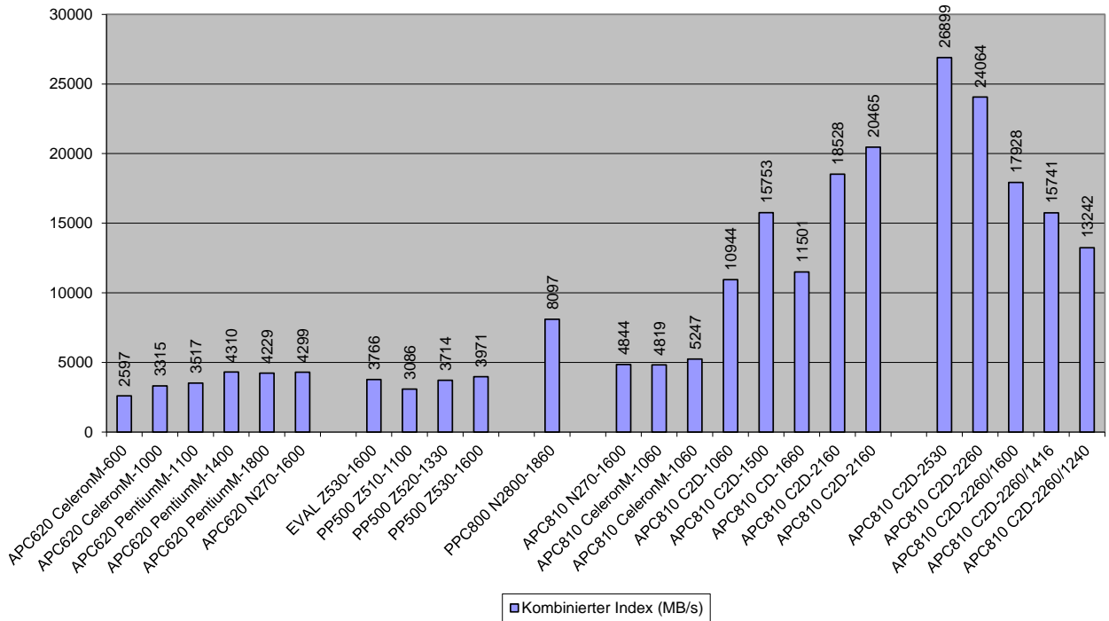
Figure 24 - Results for Sisoft Sandra Pro Business 2007, cache and memory bandwidth
