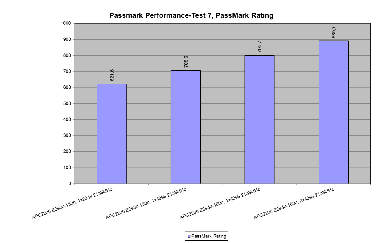
Figure 106: Results for Passmark Performance Test 7.0, Passmark Rating – APC2200/PPC2200
