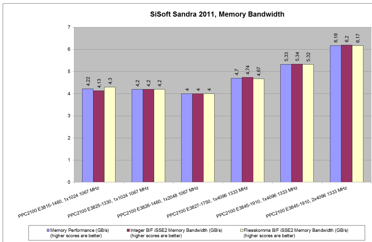
Figure 71: Results for SiSoft Sandra 2011, Memory Bandwidth – APC2100/PPC2100
